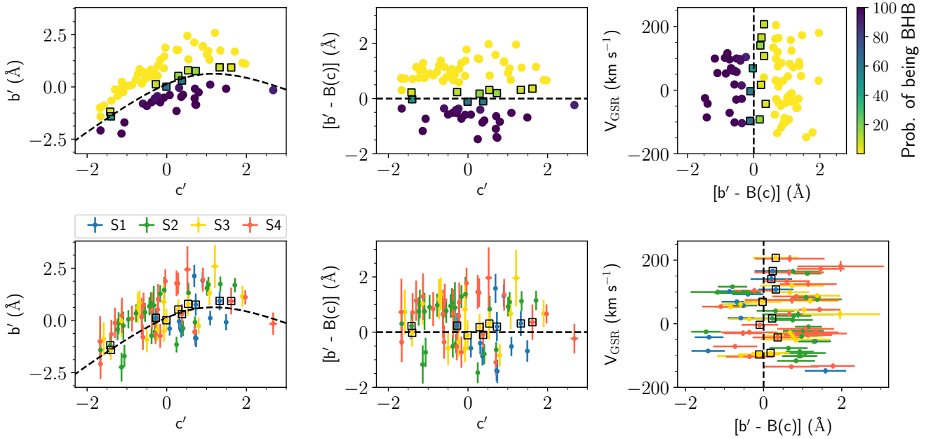
Figure 3. Stellar classification among BHB and BS stars from our FORS2 observations. The top row shows the target stars colour-coded by to the probability of being classified as BHBs. At the bottom row, the stars are colour-coded according to the substructure they tentatively belong to: blue for S1, green for S2, yellow for S3 and red for S4. Left panels show the b' and c' coefficients from the Sérsic profile, and the boundary derived based on SDSS data. In the middle panels, the c' coefficient and the difference between the b' parameter and the corresponding b' from equation 3 is shown. The rightmost panels present [b' - B(c)] against V_{\text{GSR}} . Stars marked with open squares are those which can be either BHB or BS as they are located just at the separation boundary between the two classes.
