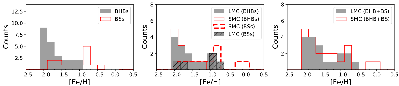
Figure 11. Metallicity distribution of BHB and BS stars in the MCs. Left: [Fe/H] distribution of BHB (grey filled bars) and BS (red unfilled bars) samples, irrespective of their possible association with the LMC or SMC. Middle: Same stars as in the left panel but divided into four subsamples: BHB and BS stars likely belonging to the LMC (grey filled and hatched bars, respectively), BHB (red unfilled bars) and BS (red dashed-line bars) stars likely associated to the SMC. Right: Metallicity distribution for the same stars according to the association to the LMC (grey filled bars) or the SMC (red unfilled bars), irrespective of their stellar classification.
