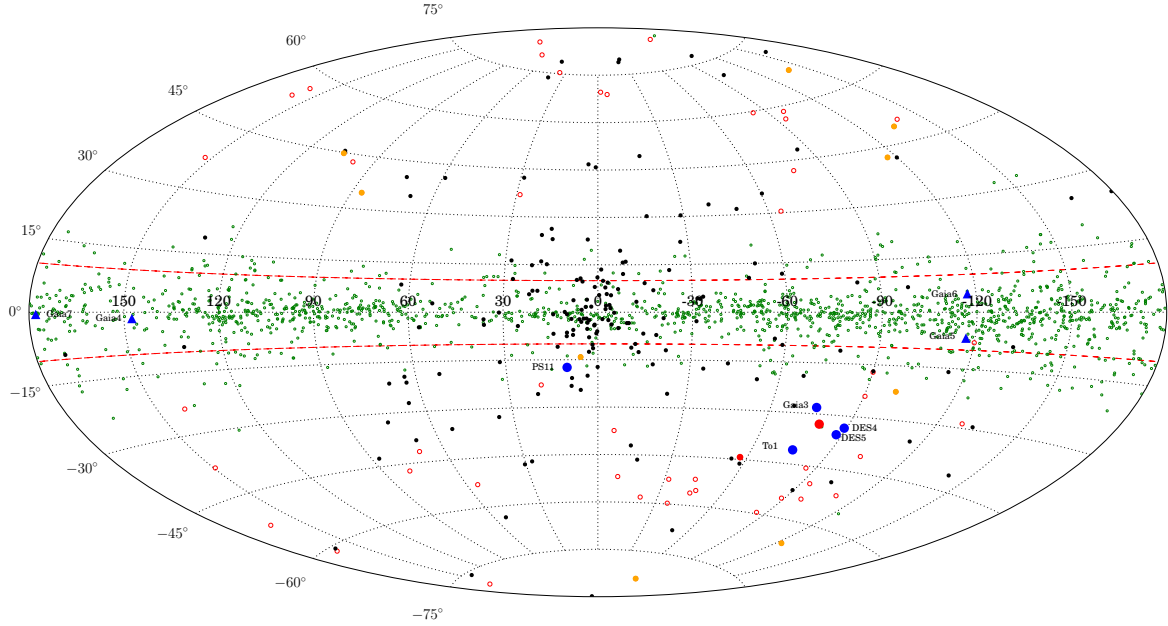
Figure 4. Spatial distribution of GCs and dwarf galaxies around the MW in galactocentric coordinates. Yellow markers shows the position of the Classical dwarfs, open red circles shows the position of other MW galaxies (from McConnachie (2012) plus Crater 2 ( Torrealba et al. 2016a ), Aquarius 2 ( Torrealba et al. 2016b ), DESJ0225+0304 ( Luque et al. 2017 ), Pictor II ( Drlica-Wagner et al. 2016 ), Virgo I ( Homma et al. 2016 ), Cetus III ( Homma et al. 2018 ), and Car II and Car III ( Torrealba et al. 2018 )), black dots the position of MW GCs ( Harris 2010 ; Belokurov et al. 2010 ; Muñoz et al. 2012 ; Balbinot et al. 2013 ; Kim & Jerjen 2015 ; Kim et al. 2015, 2016 ; Laevens et al. 2015 ; Weisz et al. 2016 ; Luque et al. 2016, 2017 ; Martin et al. 2016 ; Koposov et al. 2017 ), and green open dots show the position of MW OCs (from Kharchenko et al. 2013 ). The new discoveries are shown in blue. The red dashed lines shows |b| = 10 deg. 4 of the new discoveries, namely, Gaia 3, DES 4 and 5, and To 1 are very close to the LMC, and likely members of its GC population. The remaining 4 systems, Gaia 4 to Gaia 7, are located well within the disk, and are likely open clusters.
