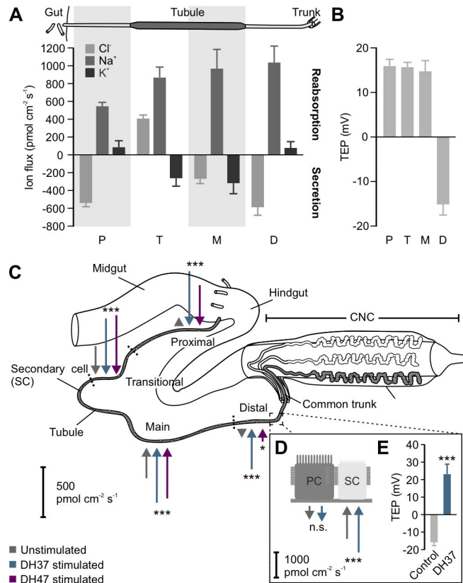
Fig. 3. Urn8 signaling modulates regional and cell-specific ion transport rates in tubules. (A) Quantitative scanning ion electrode technique (SIET) data showing Cl - , Na + and K + fluxes in the proximal (P), transitional (T), main (M) and distal (D) regions of the 'free' tubules from T. molitor . The relative length of the different functional regions of the tubule is not drawn to scale. Positive values indicate ion reabsorption (from tubule lumen to hemolymph) and negative values indicate secretion (from hemolymph to tubule lumen). (B) Transepithelial potential (TEP) voltage differences in the functionally distinct regions. (C) Schematic diagram summarizing regional and cell-specific effects of DH37 and DH47 stimulation on K + secretion in all four regions of the tubule as measured by SIET. Arrows directed towards the tissue denote net secretion while arrows directed outward indicate reabsorption. The length of the arrows corresponds to the average ion flux in each region. Both DH37 and DH47 increase net K + secretion in all four regions. CNC , cryptonephredial complex . (D) Cell-specific measurements indicate that DH37-induced changes in K + secretion are likely mediated by the SCs, which (E) reverses the lumen-negative potential in the distal segment. All data are presented as mean \pm SEM. Significant difference in K + flux from unstimulated conditions was tested using paired-sample t -test.
