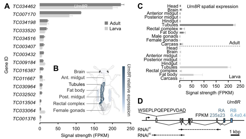
Fig 1. Transcriptomic mapping of GPCR gene expression in Malpighian tubules of Tribolium castaneum . (A) RNAseq analyses listing transcript abundance (fragments per kilobase of exon model per million reads mapped; FPKM) of all genes predicted to encode a GPCR with significantly higher expression in larval and adult MTs relative to the whole larva and adult animal, respectively. From this list TC034462 shows the highest expression, which we propose to name Urn8R . (B) Anatomical map of adult T. castaneum with superimposed heat-map of Urn8R expression across different tissues. (C) The spatial expression pattern of Urn8R indicates that it almost exclusively expressed in tubules of both larvae and adults. (D) Exon map of the Urn8R gene. The receptor is predicted to be expressed in two isoforms with -RA (235±23 FPKM) showing much higher expression than -RB (6.4±0.4 FPKM). The amino acid sequence used to raise an anti- Urn8R specific antibody, as well as the sequences targeted for RNAi knock down (RNAi #1 : bp 279-896; RNAi #2 : bp 52-273) are indicated. RNAi #1 produced the most effective knockdown (87%±0.04 SEM; n=5) and was therefore used for all subsequent experiments.
