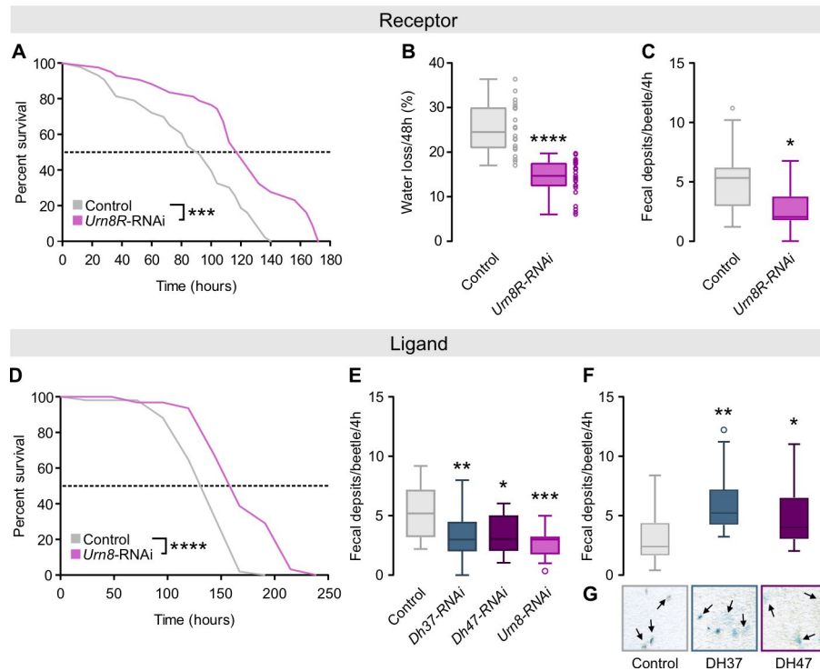
Fig. 6. Urn8 signaling regulates systemic water balance. (A) Kaplan-Meier survival function of control (dsRNA targeting beta-lactamase , amp R ) and Urn8R silenced animals. Urn8R knockdown animals survive significantly longer than controls during desiccation stress (RH 5%; log-rank test, n=43). (B) Gravimetric analyses of control and Urn8R depleted animals. Desiccation-induced water loss is significantly reduced in Urn8R knockdown animals compared to control (unpaired Student's t -test; n=22-25). (C) Defecation rate of Urn8R silenced animals is significantly lower than that of controls (unpaired Student's t -test; n=18). (D) Kaplan-Meier survival function of Urn8 silenced animals. Urn8 knockdown animals survive significantly longer than controls during desiccation stress (RH 5%; log-rank test, n=34-53). (E) Defecation rate of Dh37 -/ Dh47 -specific as well as Urn8 knockdown animals are significantly reduced relative to controls (one-way ANOVA; n=19-22). (F) Injection of DH37 or DH47 peptides (final concentration app. 10^{-7} M) into Urn8 depleted animals induce a significant increase in the number of BDP-labelled excreta produced compared to buffer-injected controls (one-way ANOVA; n=37). (G) Representative images of excreta produced in (E). DH37 or DH47 injection also results in lighter, less concentrated deposits and in increased fluid excretion (arrows) relative to controls.
