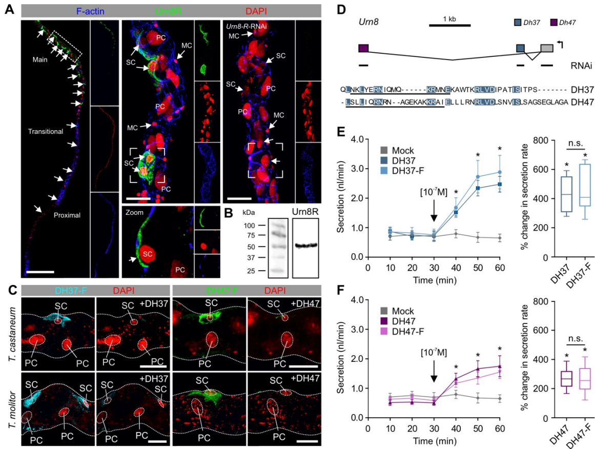
Fig 2. The Urn8 receptor localizes to a secondary cell type in MTs and is activated by its endogenous ligands DH37 and DH47. (A) Subcellular localization of Urn8R in the T. castaneum MT showing exclusive expression to the basolateral membrane of a small-nucleated secondary cell type (SC; small arrows); there are 53 \pm 2 ( n=8 ) SCs per tubule. MTs from animals injected with dsRNA targeting the Urn8 receptor ( Urn8R-RNAi ) showed a complete loss of immunoreactivity confirming specificity of the antibody. (B) Western blot analysis of protein extracts from T. castaneum tubules showing that the anti-Urn8R antiserum recognizes a protein of a size of app. 50-55 kDa, consistent with the predicted size of the receptor (=51.6 kDa for the dominant -RA isoform, arrow). (C) Application of fluorophore-coupled receptor agonists DH37-F and DH47-F ( 10^{-7} M) to T. castaneum and Tenebrio molitor MTs. Specific and displaceable binding to the SCs is observed, as competitive inhibition with 'cold' unlabeled ligands DH37 and DH47 ( 10^{-5} M) almost fully abolished the fluorescent signal. (D) Exon map of the T. castaneum Urn8 ( TC030022 ) gene encoding the two predicted Urn8 ligands, DH37 and DH47, produced by alternative splicing of two separate exons to a common 5' exon encoding the signal peptide (12). The regions targeted for RNAi knockdown (either common or ligand-specific sequences) and the amino acid sequences used to raise ligand-specific antibodies are indicated. Amino acids shared between the two ligands are highlighted in blue. (E-F) Both the labelled and unlabeled ligands significantly stimulate fluid secretion rates compared to unstimulated (artificial hemolymph only; mock) MTs of T. molitor (paired-sample t -test, n=10 ). Black arrows indicate time of peptide application. DH37 induces a significantly higher percent change in fluid secretion compared to DH47 (unpaired-sample t -test, n=10 ). Fluorophore coupling does not significantly affect the functional efficacy of the peptides (unpaired-sample t -test, n=10 ). Values are expressed as mean \pm SEM.
