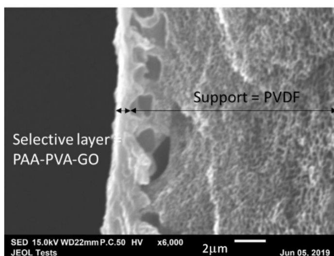
Figure 3. SEM images of a cross-section of polyallylamine (PAA)-poly(vinyl alcohol) (PVA)-graphene oxide (GO) membrane.
