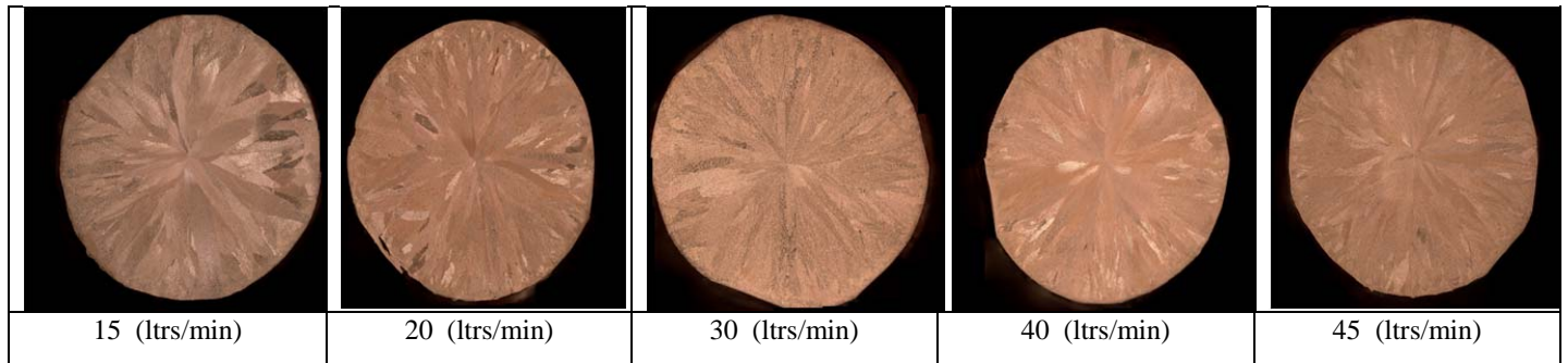
Fig.3 Comparison grain structure of CuSnP samples
