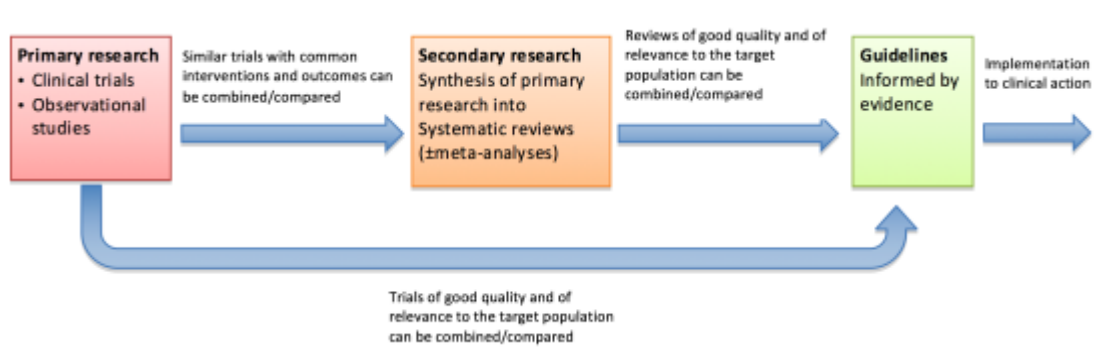
Figure 2. The flow of evidence creation from trials to guidelines. Pre-trial research and implementation findings informing future research have been omitted for simplicity.
