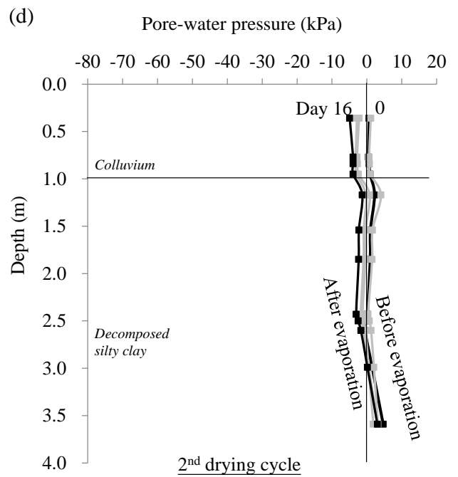
7 Figure A5. Measured instantaneous profiles of (a) VWC and (b) PWP of colluvium and decomposed 8 silty clay during the 1 st drying cycle; and (c) VWC and (d) PWP during the 2 nd drying cycle reported 9 by Ng et al. (2011)
