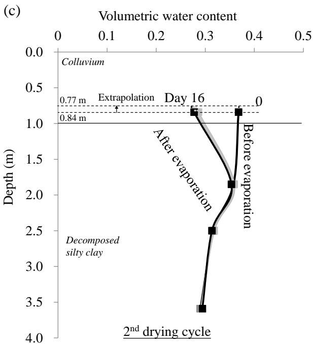
7 Figure A5. Measured instantaneous profiles of (a) VWC and (b) PWP of colluvium and decomposed 8 silty clay during the 1 st drying cycle; and (c) VWC and (d) PWP during the 2 nd drying cycle reported 9 by Ng et al. (2011)
