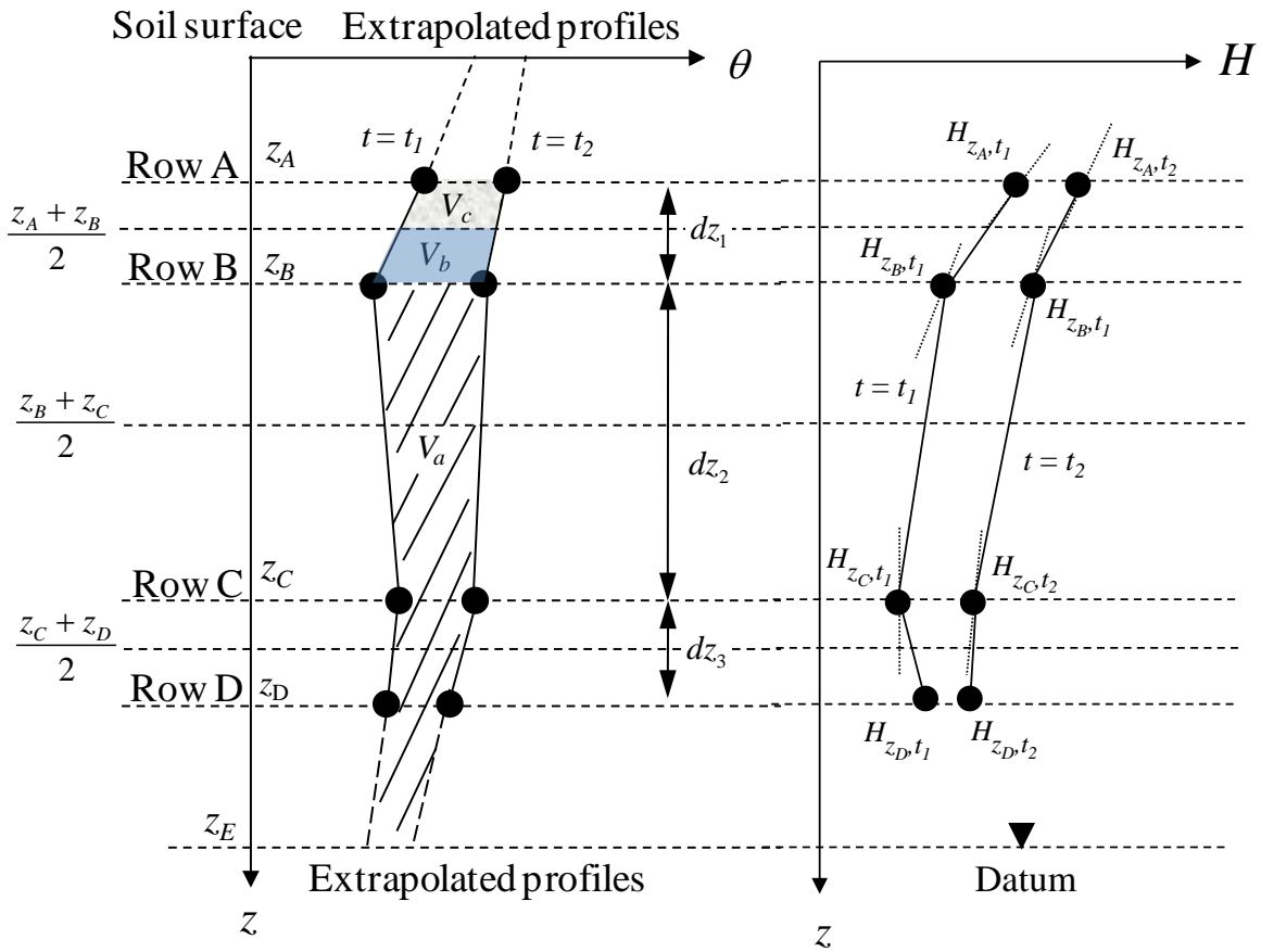
Figure 1. Arbitrary instantaneous profiles of VWC ( \theta ) and hydraulic head ( H ) at elapsed times, t = t_1 and t_2 , along a one-dimensional soil column
