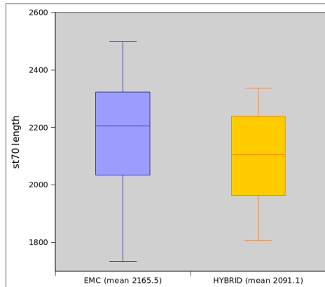
Fig. 3: Comparison of the tours found by EMC and Hybrid searches on instance st70
