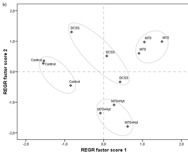
635 Figure 4. Component plot (a) and factor score plot (b) of the multivariate Principal 636 Components Analysis of lipid peroxidation (LPOprot), antioxidant enzymes (Catalase 637 (CAT), glutathione-s-transferase (GST), superoxide dismutase (SOD), total glutathione 638 peroxidase (GPxTot), Selenium dependent glutathione peroxidase (GPxSe)) and total 639 HUFA (n-3 and n-6 series) of enriched Artemia nauplii with commercial emulsion 640 DCSS, M70 emulsion, M70 emulsion in combination with an external antioxidant, HYT 641 (M70+HYT treatment) and non-enriched Artemia from Experiment 2.
