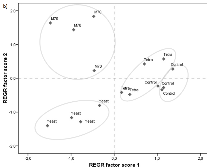
617 Figure 2. Component plot (a) and factor score plot (b) of the multivariate Principal 618 Components Analysis of lipid peroxidation (LPOprot) and antioxidant enzymes 619 (Catalase (CAT), glutathione-s-transferase (GST), superoxide dismutase (SOD), total 620 glutathione peroxidase (GPxTot), Selenium dependent glutathione peroxidase (GPxSe))
