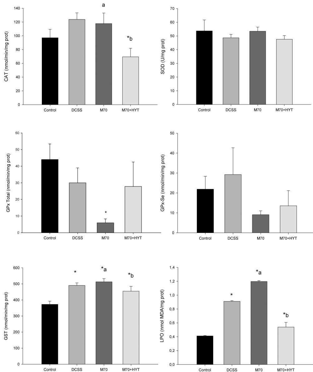
624 625 Figure 3. Activity of Catalase (CAT), superoxide dismutase (SOD), total glutathione 626 peroxidase (GPx Total), Selenium dependent glutathione peroxidase (GPx Se-dep), 627 glutathione-s-transferase (GST) and lipid peroxidation (LPO) in whole body of non- 628 enriched Artemia nauplii and Artemia nauplii enriched with commercial emulsion 629 DCSS, M70 emulsion and M70 emulsion in combination with an external antioxidant 630 HYT, M70+HYT treatment. Asterisk shows statistical differences between the 631 treatment and the control group (Dunnett test) and lowercase letter superscript shows 632 statistical differences between M70 and M70+HYT treatment (Student t-test).
