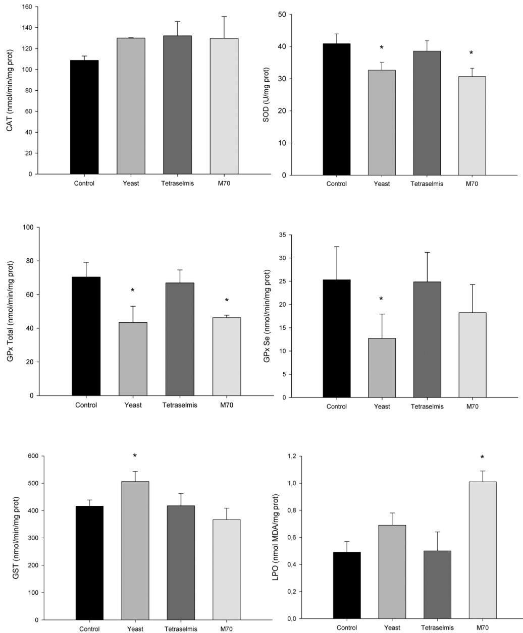
609 Figure 1. Activity of Catalase (CAT), superoxide dismutase (SOD), total glutathione 610 peroxidase (GPx Total), Selenium dependent glutathione peroxidase (GPx Se-dep), 611 glutathione-s-transferase (GST) and lipid peroxidation (LPO) in whole body of Artemia 612 nauplii enriched with M70 emulsion, Tetraselmis suecica algae, yeast ( Saccharomyces 613 cerevisiae ) and non-enriched Artemia . Asterisk shows statistical differences between the 614 different treatments and the control group (Dunnnett test).
