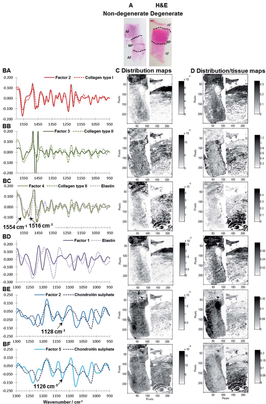
Fig. 6 H&E of non-degenerate (left) and degenerate (right) human IVDs (A). MCR-ALS calculated spectral profiles of Factor 2 (950–1600 \text{cm}^{-1} , modelled with five factors) vs. reference profiles of collagen type I (BA), Factor 3 (950–1600 \text{cm}^{-1} , modelled with five factors) vs. collagen type II (BB), Factor 4 (950–1600 \text{cm}^{-1} , modelled with five factors) vs. collagen type II and elastin (BC), Factor 1 (950–1300 \text{cm}^{-1} , modelled with five factors) vs. elastin (BD), Factor 2 (950–1300 \text{cm}^{-1} , modelled with five factors) vs. chondroitin sulphate (BE) and Factor 5 (950–1300 \text{cm}^{-1} , modelled with five factors) vs. chondroitin sulphate (BF) as well as corresponding distribution maps (C) and distribution/tissue maps (D) of non-degenerate (left) and degenerate (right) human IVD sections.
