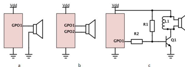
Figure 1. Conventional architectures to drive an ultrasonic transmitter (GPO-General purpose output pin of the microcontroller)
