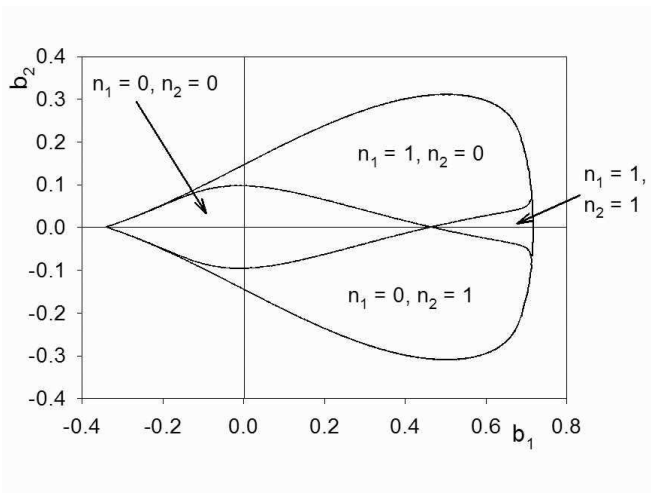
FIG. 17: Solution space for \mathfrak{su}(3) solitons with \Lambda = -1 . Where we find solutions, the numbers of zeros of the gauge field functions are indicated. Elsewhere in the parameter space we do not find solutions. We now have a much larger region of solutions in which both gauge field functions have no zeros.
