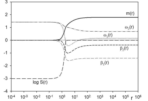
FIG. 15: Typical \mathfrak{su}(3) soliton solution, with \Lambda = -0.1 , b_1 = 0.35 and b_2 = 0.115 . The gauge field function \omega_1(r) has two zeros, while \omega_2(r) has no zeros.
