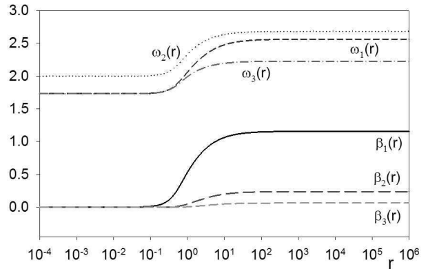
FIG. 18: Typical \mathfrak{su}(4) soliton solution, with \Lambda = -10 , b_1 = -1.2 , b_2 = -0.1 and b_3 = -0.01 . We plot just the auxiliary functions \beta_k(r) and the gauge field functions \omega_j(r) . In this example, all three gauge field functions have no zeros. Note that \beta_3(r) is not identically zero, it monotonically increases to 6.41 \times 10^{-2} as r \rightarrow \infty .
