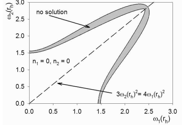
FIG. 14: Solution space for \mathfrak{su}(4) EYM black holes with \Lambda = -10 , r_h = 1 and \omega_1(r_h) = \omega_3(r_h) . The shaded region indicates those values of the parameters \omega_1(r_h) , \omega_2(r_h) for which the constraint (3.13) is satisfied, but for which we find no black hole solutions. In this case, for all the black hole solutions we find, all three gauge field functions have no zeros. We have also plotted the dashed line 4\omega_1(r_h)^2 = 3\omega_2(r_h)^2 , on which lie embedded \mathfrak{su}(2) solutions.
