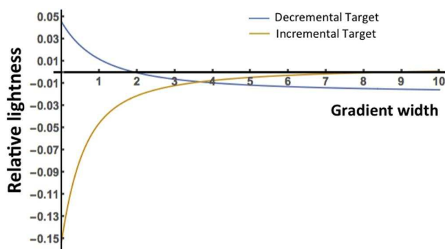
Fig. 8. 1D computer simulation of the phantom illusion based on Rudd's edge integration model. Contrast gain control was assumed to occur between pairs of Stage 1 and Stage 2 oriented contrastdetecting neurons
