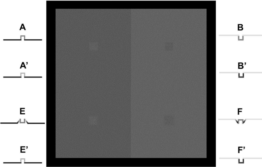
Fig. 5. Configuration 2, display pairs AB atop display pair EF. On the side of the displays are depicted the luminance profiles. Profiles A ~ , B ~ , E ~ , and F ~ epitomize the perceptual phenomenal outcome as reported by the observers.
