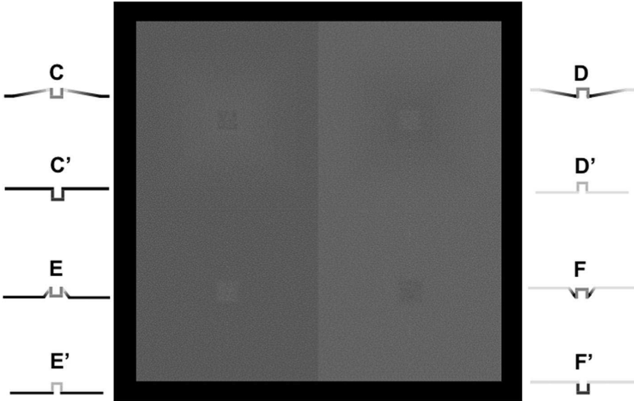
Fig. 6. Configuration 3, display pairs CD atop display pair EF. On the side of the displays are depicted the luminance profiles. Profiles C ~ , D ~ , E ~ , and F ~ epitomize the perceptual phenomenal outcome as reported by the
