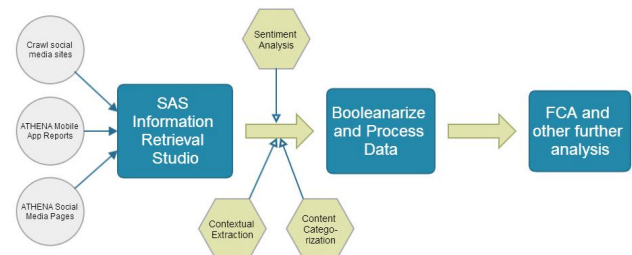
Fig. 3: The data processes within the CIPC
