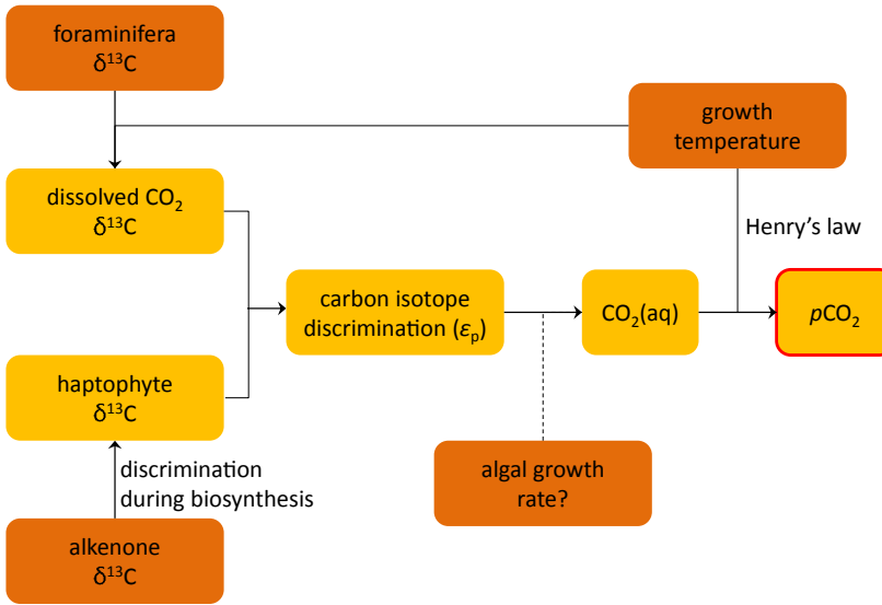
Figure 4 A guide to reconstructing ancient pCO 2 levels from the determination of alkenone and foraminiferal δ 13 C values. Quantities in orange boxes are things that must be measured or inferred and those in yellow are calculated.
