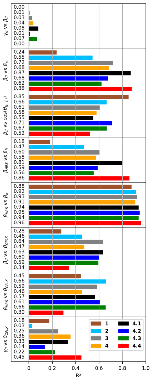
Figure 7. Linear correlation analyses between pairs of molecular properties. The nonlinear optical properties are represented by \beta_x , \beta_{II} , \beta_{HRS} , and \gamma_{II} . \theta_{(\mu, \beta)} is the angle between the \mu and \beta vectors. \theta_{CPLX} represents the angle between the two cations.
