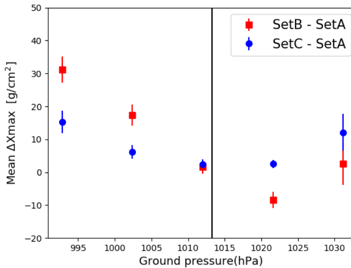
Figure 2: Difference in mean X_{\max} as a function of ground pressure. The total sample contains 123 air showers recorded at LOFAR. The black line denotes the U.S standard atmospheric pressure.
