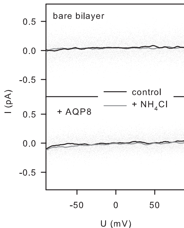
FIGURE 2. Exclusion of \text{NH}_4^+ transport by AQP8. The current voltage characteristics of bare lipid bilayers and bilayers reconstituted with AQP8 are not altered by the hundredfold augmentation of the \text{NH}_4\text{Cl} bulk concentration. A voltage ramp (duration 3 min) was applied in the interval from -90 to +90 mV. The current was measured with a frequency of 100 Hz and then filtered at 0.3 Hz (compare "Experimental Procedures"). The resulting data cloud is plotted. The spline lines were obtained by applying a local smoothing technique (100 intervals) using polynomial regression and weights computed from the Gaussian density function (SigmaPlot). The similarity of their slopes indicates that AQP8 excludes other ions as well. Membrane and buffer composition were as in Fig. 1.
