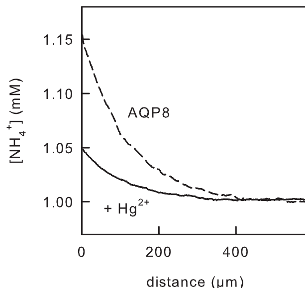
FIGURE 4. Inhibition of AQP8 mediated \text{NH}_3 transport by \text{Hg}^{2+} . Reconstitution of AQP8 in a protein:lipid ratio of 1:120 resulted in a \text{NH}_3 permeability of 50 \mu\text{m/s} . 1 mM \text{Hg}^{2+} reduced the permeability to that of a bare bilayer (here to 15 \mu\text{m/s} ). The corresponding transmembrane \text{NH}_3 fluxes were 0.2 and 0.06 \text{nmol cm}^{-2} \text{s}^{-1} in the absence and presence of \text{Hg}^{2+} , respectively. The trans and cis \text{NH}_4\text{Cl} concentrations in the bulk were equal to 1 and 80 mM, respectively. Buffer composition was as in Fig. 1.
