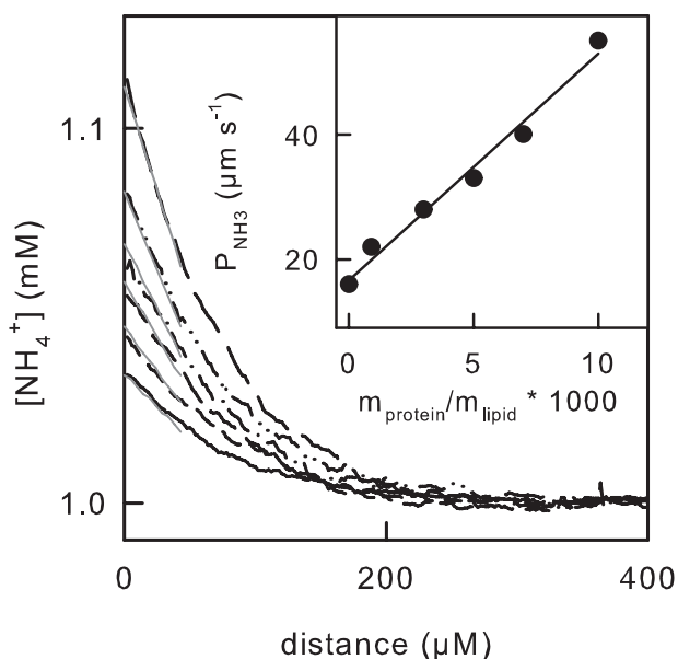
FIGURE 5. NH 3 membrane permeability as a function of AQP8 membrane abundance. The trans and cis NH 4 Cl concentrations in the bulk were equal to 1 and 80 mM, respectively. In the absence of the protein ( spline line ), a modest increase in the cis NH 4 + concentration was observed in the immediate membrane vicinity. Upon reconstitution of AQP8, the augmentation of NH 4 + concentration adjacent to the membrane became more pronounced. The more protein was reconstituted, the higher was the concentration polarization. The gray lines represent concentration profiles generated by the theoretical model of weak base diffusion (Equations 1–3 and Reactions 1 and 2). The P_{NH_3}^M values used to calculate the theoretical curves are plotted in the inset as a function of the protein:lipid ratio. Buffer composition was as in Fig. 1.
