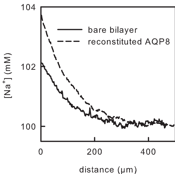
FIGURE 1. Water transport by AQP8. Reconstitution of AQP8 (protein:lipid = 1:100) augmented water permeability of bare lipid bilayers (cholesterol: E. coli lipid extract: sphingomyelin = 3:2:1) from 11 to 27 \mu\text{m/s} . Water permeability was calculated from the dilution of \text{Na}^+ ions shown as a function of the distance to the membrane. Osmotic water flux was induced by 1 M urea. The buffer contained 20 mM MES, 100 mM NaCl, 1 mM \text{NH}_4\text{Cl} , pH 6.0.
