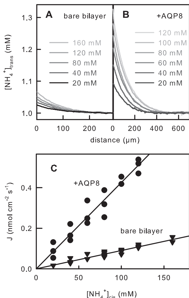
FIGURE 3. \text{NH}_3 flux J as a function of the transmembrane \text{NH}_4\text{Cl} concentration gradient. The \text{NH}_4^+ concentration in the trans compartment was measured by scanning microelectrodes as a function of the distance to the membrane. A , representative concentration profiles visualizing \text{NH}_3 diffusion through a bare lipid bilayer made of a lipid mixture (cholesterol: E. coli lipid extract: sphingomyelin = 3:2:1). B , representative concentration profiles showing \text{NH}_3 diffusion through reconstituted AQP8. For membrane formation the same lipid composition as in panel A was used. The protein:lipid ratio was 1:50. C , \text{NH}_3 flux at different \text{NH}_4^+ bulk concentrations in the cis compartment. J_{\text{NH}_3} and P_{\text{NH}_3} were calculated using the analytical model of weak base diffusion (Equations 1–3 and Reactions 1 and 2). The regression lines correspond to \text{NH}_3 permeabilities of 16 and 105 \mu\text{m/s} for bare and AQP8-containing bilayers, respectively. The buffer solution contained 20 mM MES, 100 mM NaCl, pH 6.0. The trans compartment contained 1 mM \text{NH}_4\text{Cl} .
