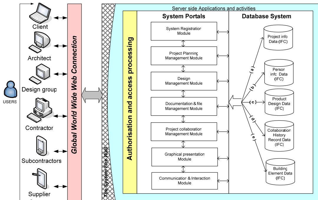
Figure 5.2: CODE system architecture, the database system headlights the five major areas in the CODE database
