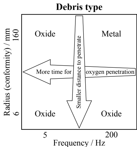
Figure 15: Debris type fretting map, identifying the nature of the debris formed during fretting as a function of contact conformity and fretting frequency. Superimposed on the map are arrows representing changes in fundamental processes associated with oxygen penetration into the contact which depend upon the parameters upon which the map is constructed.
