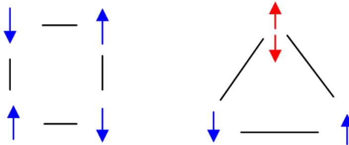
Figure 81: Demonstration of frustration in a system. The red arrow can be in either state and the energy of the system would be the same.
