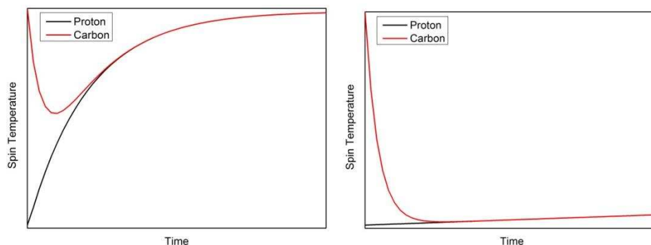
Figure 29: Schematic representation of the spin temperatures of a sample during thermal mixing. The graph to the left is a case when the T_1 time of the protons is short compared to the time require for thermal mixing, while the graph to the right is when the T_1 of the protons is long compared to the required mixing time.
