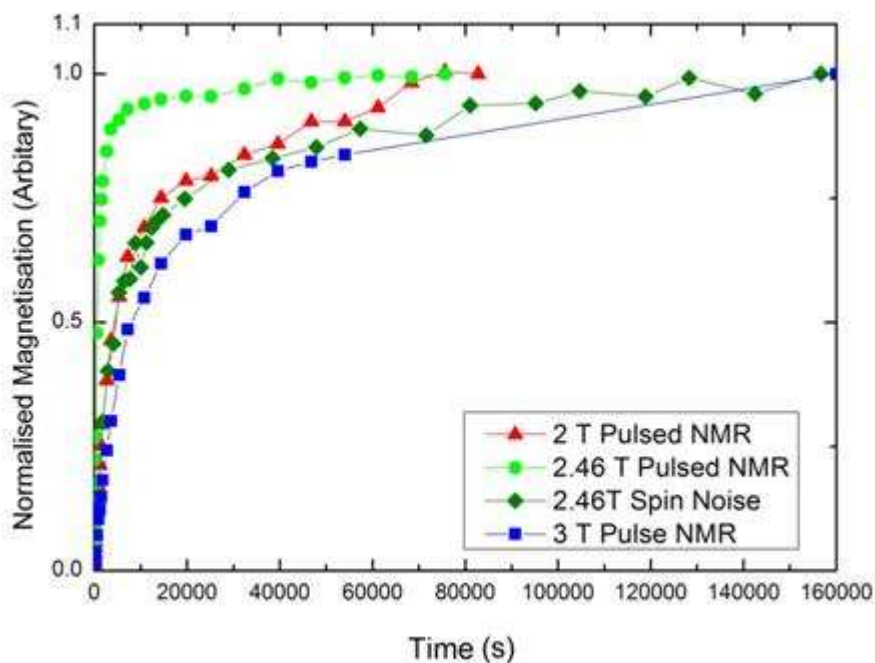
Figure 35: Proton T_{1/2} measured using spin noise measurements on a 20:1 WG 2 M NaAC:CuO sample at 20 mK
