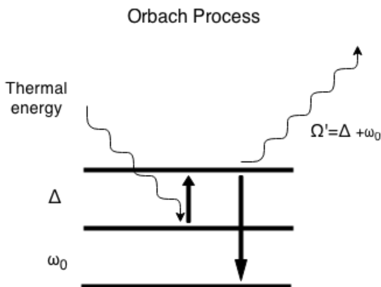
Figure 31: Schematic of the Orbach process. Thermal energy promotes the spin to a higher energy level before it relaxes to a lower energy level releasing a phonon.
