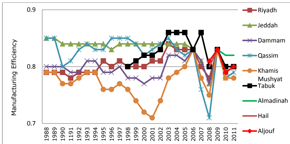
Figure 1.4: Manufacturing yield for GSFMO mills (1988-2011)
