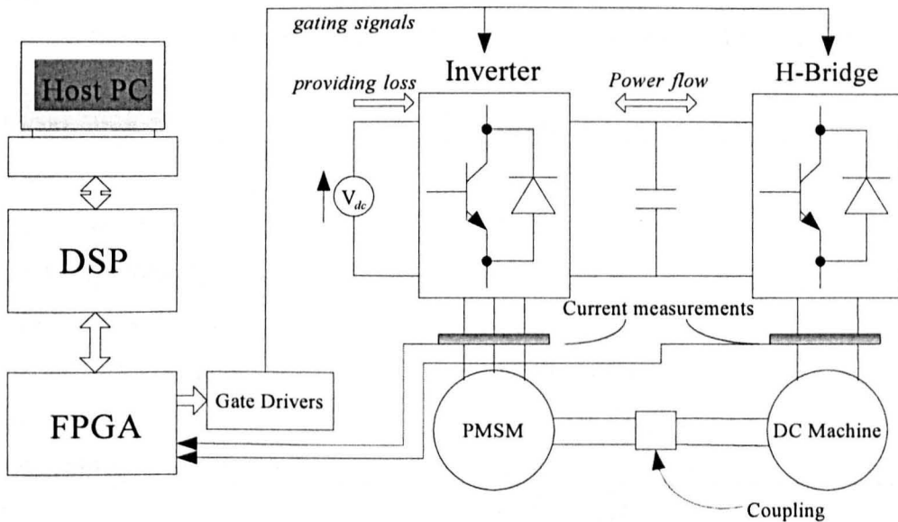
Figure 4.1: The overall system of the test rig
