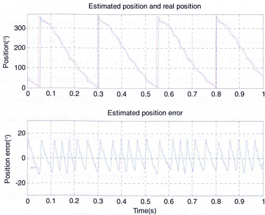
Figure 5.16: Results of armature compensation by predefined offset at 50A (56%)
