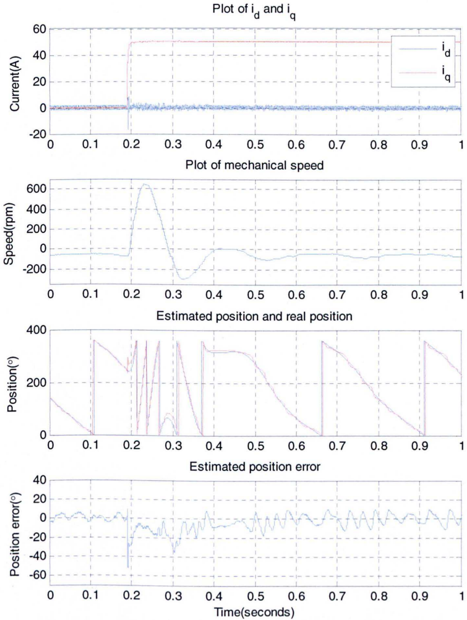
Figure 6.16: Torque transient, 0-50A (56%), (2000 ± 328) Hz random injection at -60rpm
