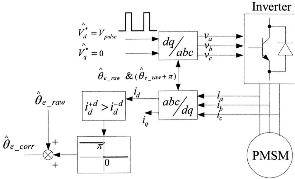
Figure 5.2: Initial polarity detection scheme
