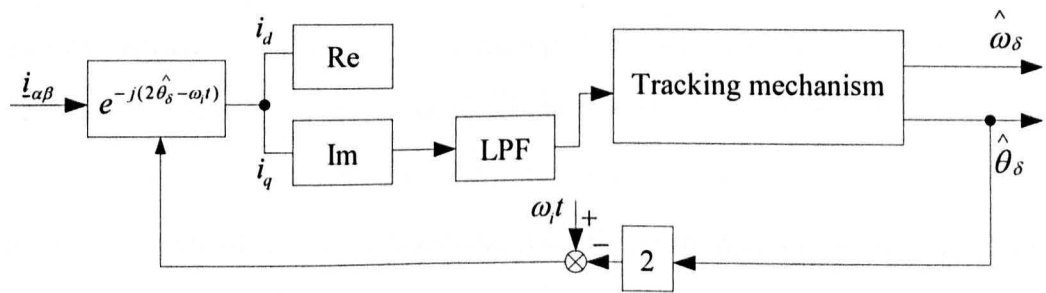
Figure 2.6: Scheme of heterodyne demodulation for \alpha\beta injection method
