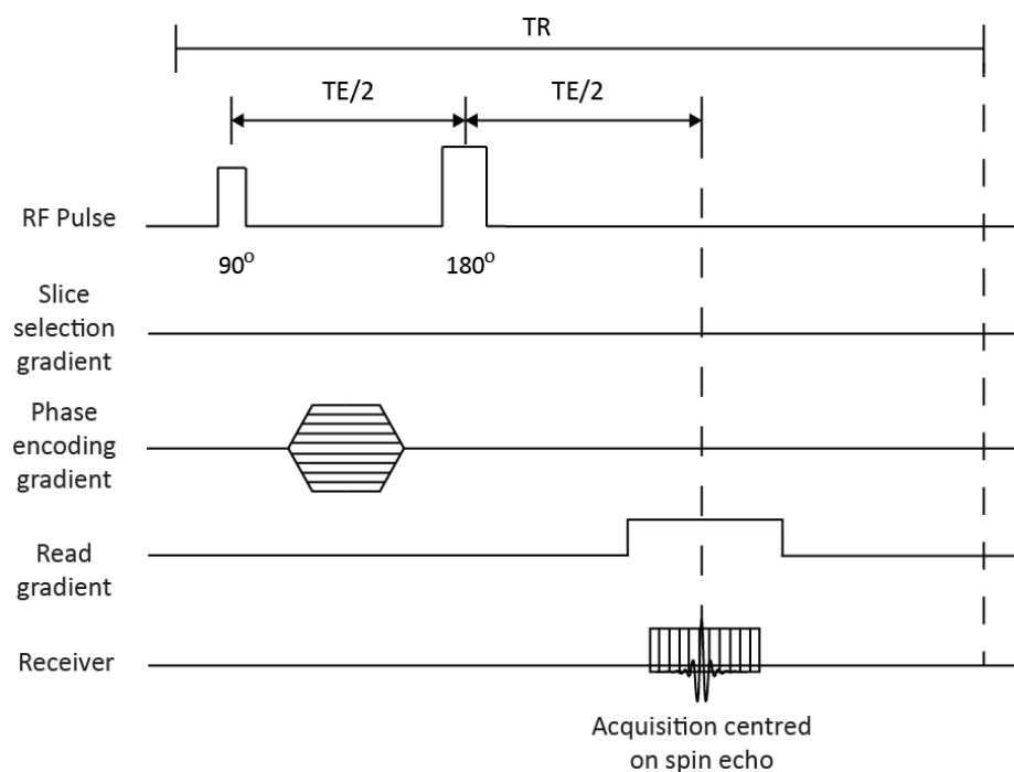
Figure 2.4 Non slice selective spin echo pulse sequence. 90^\circ rectangular RF pulse followed by a 180^\circ rectangular refocusing pulse at TE/2 with formation of the spin echo at TE. Application of the read gradient with opening of the acquisition window centred on the spin echo. After time TR, the process is repeated with different strengths of the phase encoding gradient. Note the length of TR is not representative and is often much longer than TE but has been reduced for ease of display.
