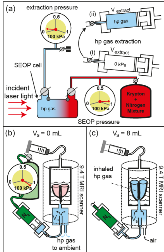
Fig. 6.1. Hp krypton-83 gas extraction and transfer from the SEOP cell in the hyperpolarizer to the lungs (ambient pressure). (a) A pre-evacuated volume V_{extract} = 790 \text{ cm}^3 in the extraction unit (i) was filled to approximately 6 kPa during hp gas extraction from the SEOP cell in the hyperpolarizer (operating at 90 – 100 kPa) (ii). (b) The extraction unit was moved to the MRI scanner and the \text{N}_2 gas operated piston pressurized the hp gas mixture to a slightly above ambient pressure. The hp gas was then pushed through connecting tubing into a storage container ( V_B ). (c) Inhalation of the hp gas was accomplished by pulling to volume V_s = 8 \text{ mL} on the ventilation syringe to expand the lung as has been previously demonstrated. Modified with permission from Fig. 1 in Appendix 1 and ref. [216].
