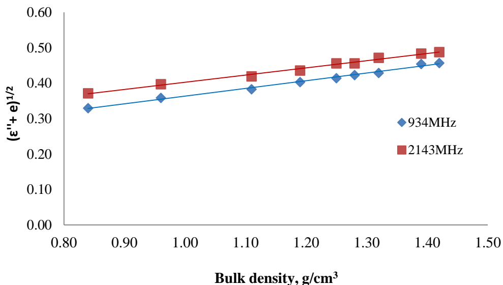
Figure A:3-21: Linear relationship between (\epsilon'' + e)^{1/2} and density for South African sample
