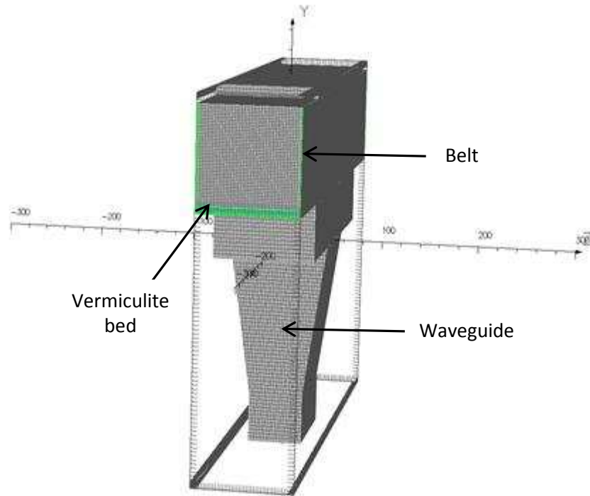
Figure 5-1: Model of the applicator with fine cubic mesh applied over it for the purposes of the FDTD simulation.
