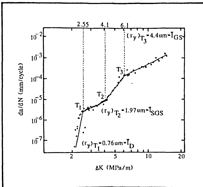
2.13 Fatigue crack growth rates in 7075-T6 alloy (107)
