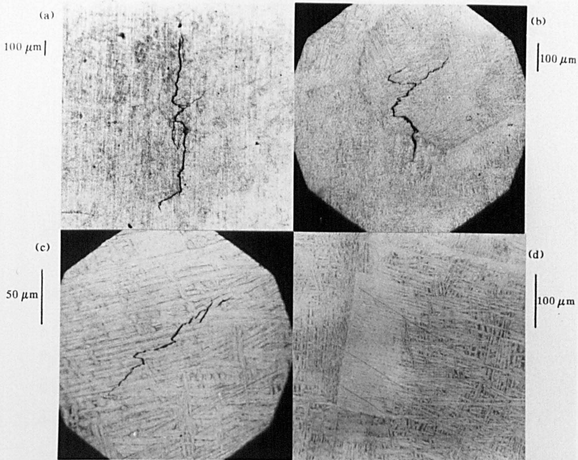
8.14 (a) - (c) Optical micrographs showing surface crack history of short crack described in figure 8.10b for 318E. (d) Optical micrograph showing slip band cracking in 318E. (a) 580000 cycles (b) 570000 cycles (c) 430250 cycles
