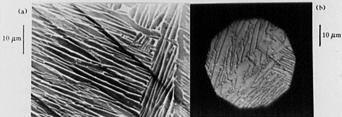
8.15 (a) Electron micrograph of slip band cracking in 550B. (b) Optical micrograph showing initiation of short fatigue crack at a prior grain boundary in 550B.
