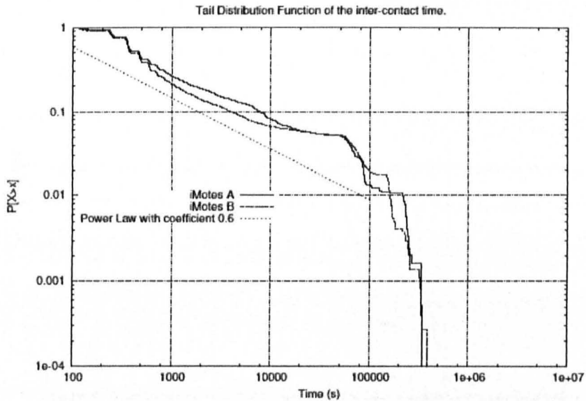
Figure A.4: Distribution of inter-contact times between iMotes and other Bluetooth devices. Experiment iMote A included nine researchers and interns working at Intel Research Cambridge, while iMote B involved twelve doctoral students and faculty comprising a research group at the University of Cambridge Computer Lab (Source [1]).
