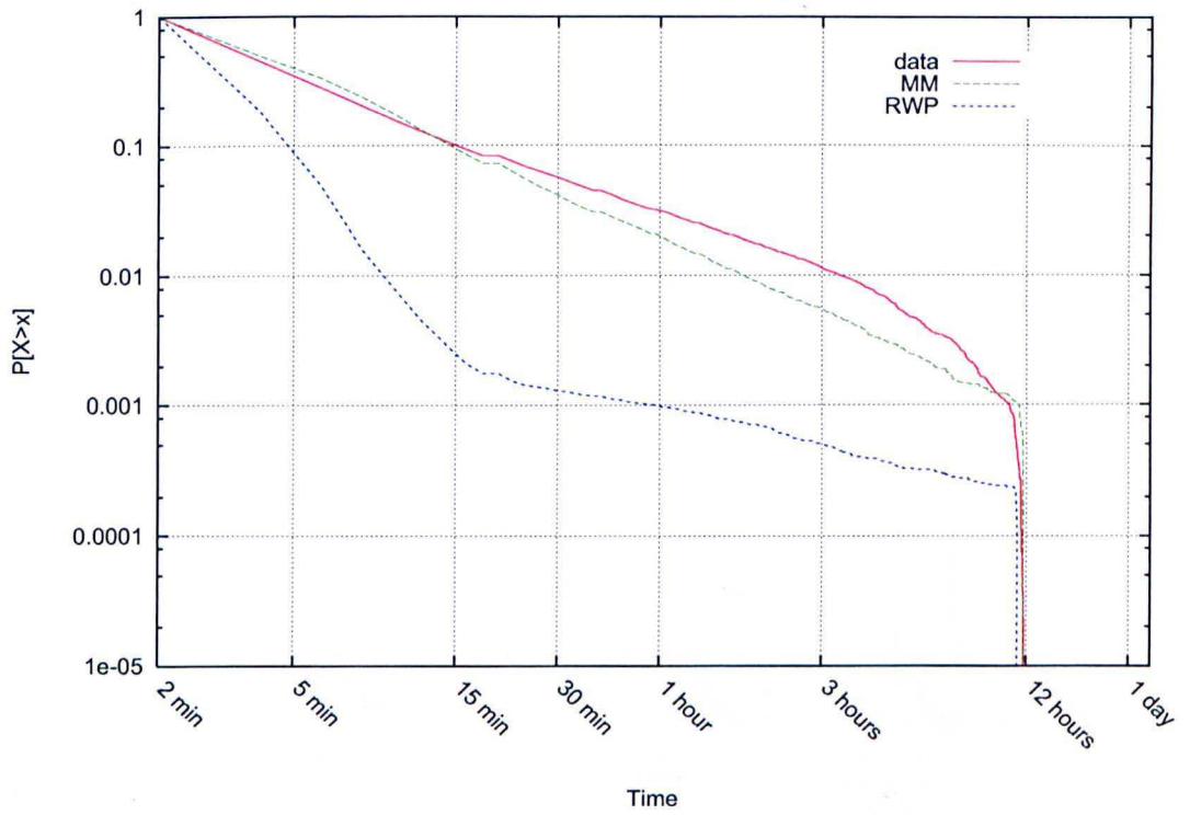
Figure 4.7: Comparison between synthetic and real traces: cumulative distributions of contact duration
