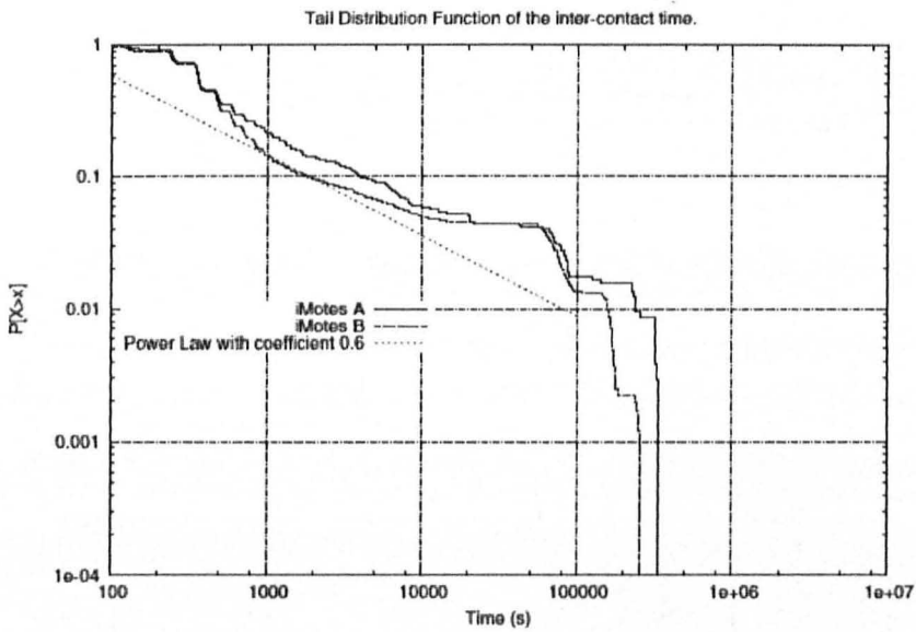
Figure A.3: Distribution of inter-contact times between iMotes. Experiment iMote A included nine researchers and interns working at Intel Research Cambridge, while iMote B involved twelve doctoral students and faculty comprising a research group at the University of Cambridge Computer Lab (Source [1]).
