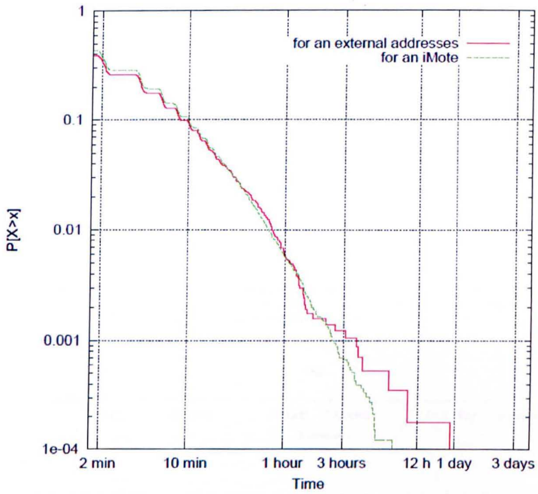
Figure A.7: Distributions of inter-contact times for pairs of nodes (Source [2]).
