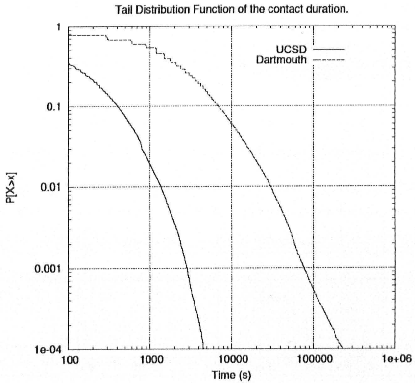
Figure A.6: Distribution of contact duration for WiFi data sets from UCSD and Dartmouth (Source [1]).
