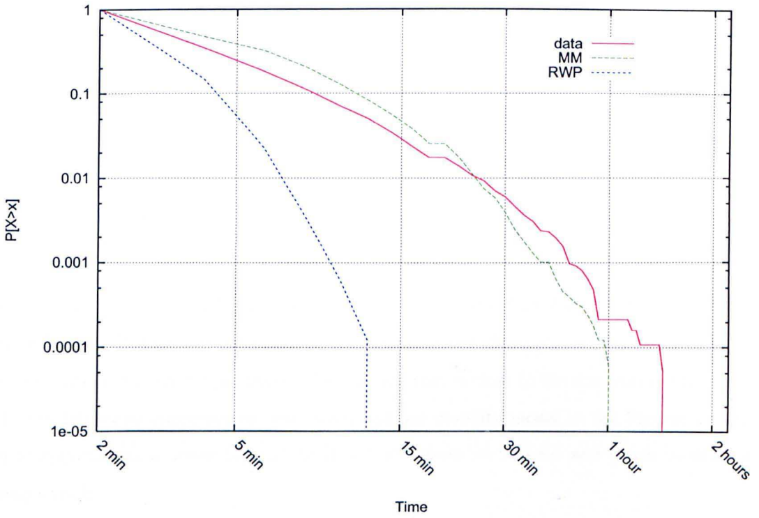
Figure 4.5: Comparison between customers' synthetic and real traces: cumulative distributions of contact duration
