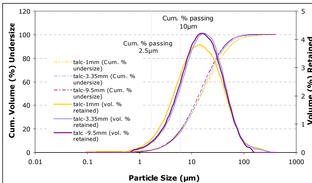
Figure 85: Particle size distribution of the talc particulate matter produced through (a) the OPT-TP and (b) the HSL-TP. The presented results correspond to average values of repeatable tests.
