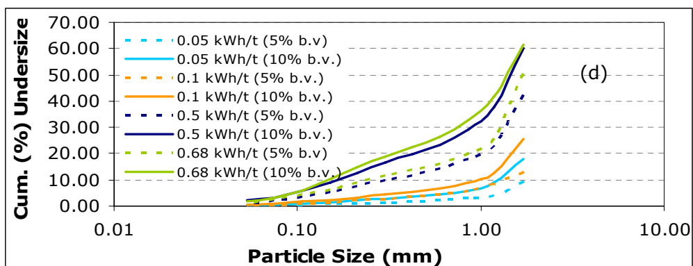
Figure 136: Particle size distribution of the copper ore particles after impact for the single fractions (a) -16+13.2mm (10% and 20% bulk volume) and (b)-8+6.7mm fractions, (c) -4+3.35mm, (d) -2+1.7mm (5% and 10% bulk volume).
