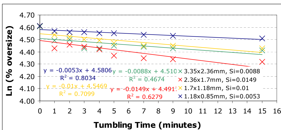
Figure 53: Natural logarithm of the percentage oversized against tumbling time for the limestone single fractions 3.35x 2.36mm, 2.36x1.7mm, 1.7x1.18mm and 1.18x0.85mm and for tumbling speed 30rpm.
