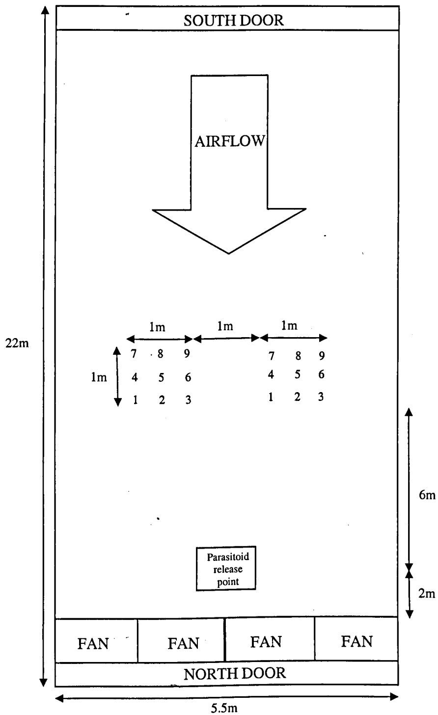
Figure 6.2 Polytunnel specifications and experimental design.
