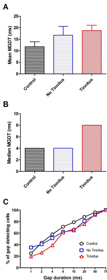
Fig. 5.11: Mean (A) and median (B) MGDs of single-units for the three different groups in response to BBN. (C) shows gap detection thresholds as a function of % of responding cells.
