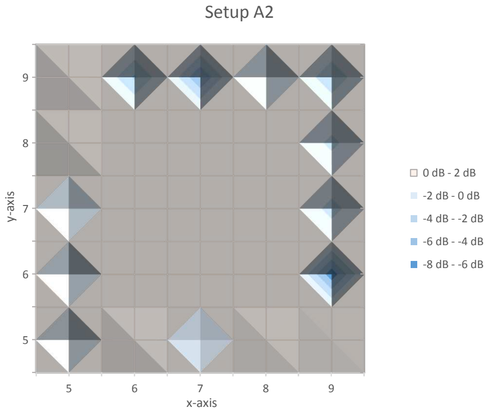
FIGURE 8-6: DIFFERENCE BETWEEN PRESENT AND EMPTY RSS VALUES FOR SETUP A2
