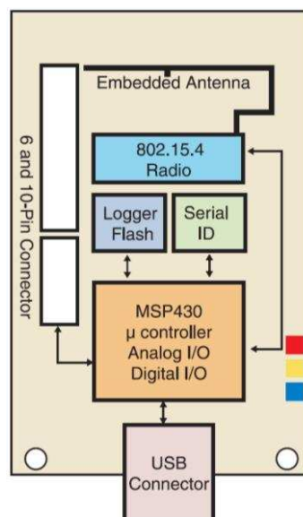
FIGURE 7-1: TELOS B BLOCK DIAGRAM [138, P.1]
