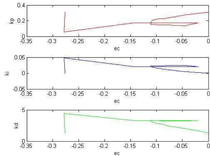
Figure 4-6 PID parameters varying based on ec
