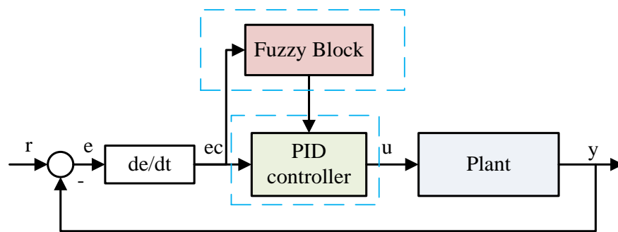
Figure 2-11 A typical fuzzy-PID controller
