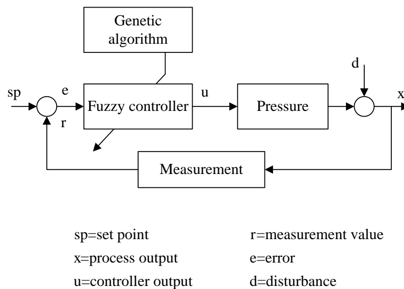
Figure 2-13 Fuzzy controller using genetic algorithm structure [303]
