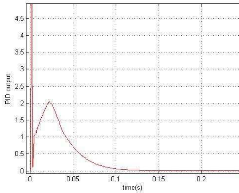
Figure 4-3 PID output response to step input
