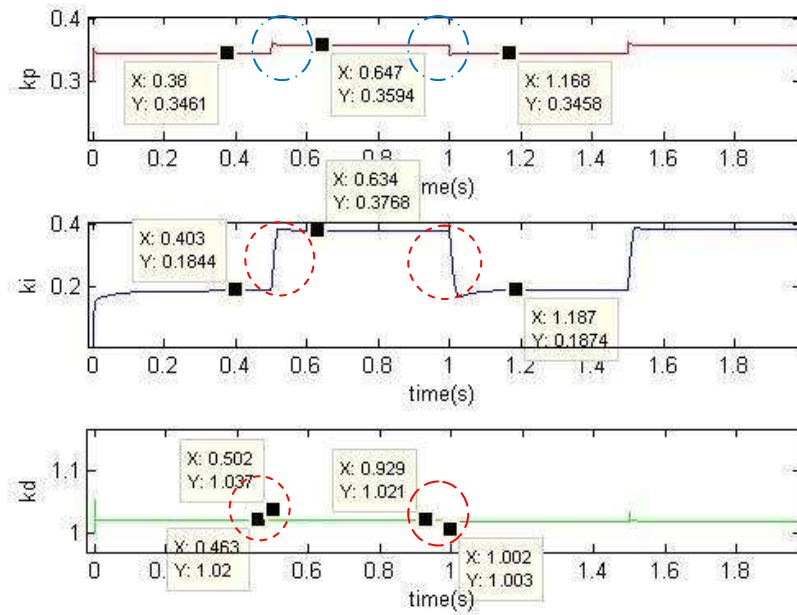
Figure 4-15 PID parameters regulating process
