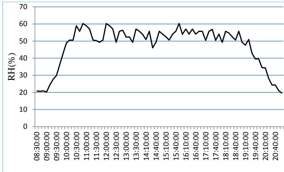
Figure 5-32 Indoor RH monitored in-Jan 2013
