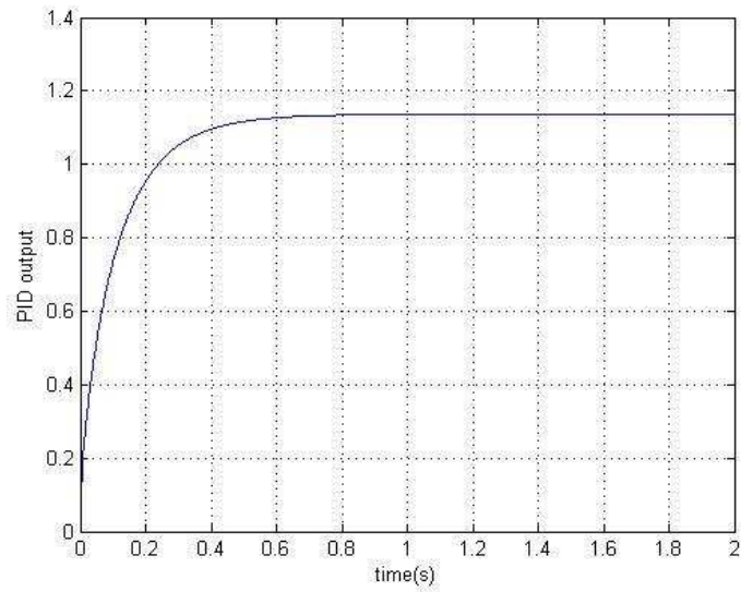
Figure 4-8 PID output response to step input
