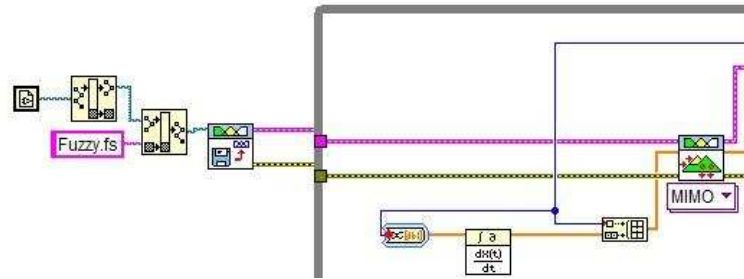
Figure 5-17 MIMO fuzzy controller
