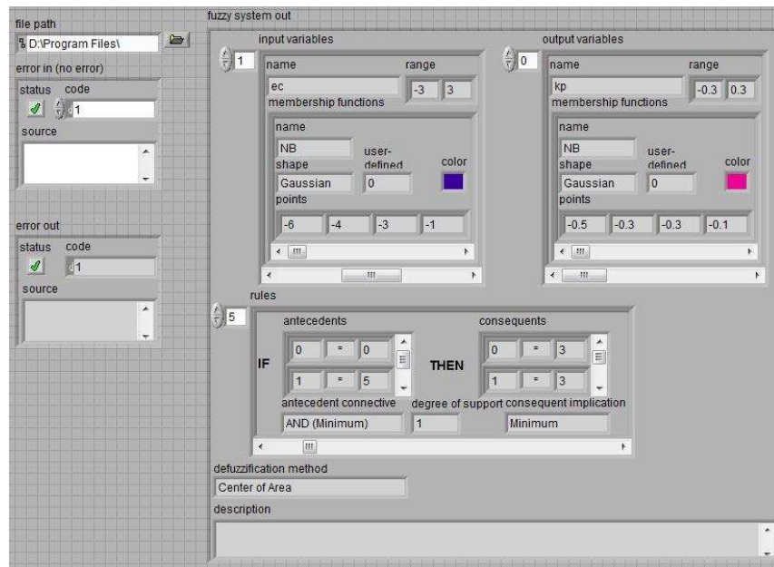
Figure 5-16 Front panel of fuzzy system load VI
