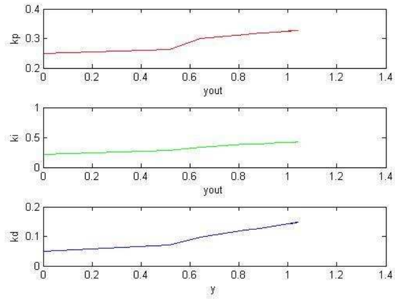
Figure 4-23 PID parameters response to system output
