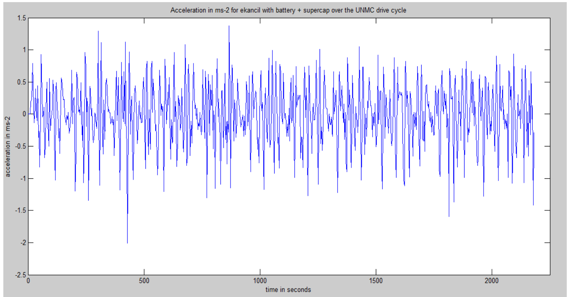
Fig 74 : Vehicle Acceleration
