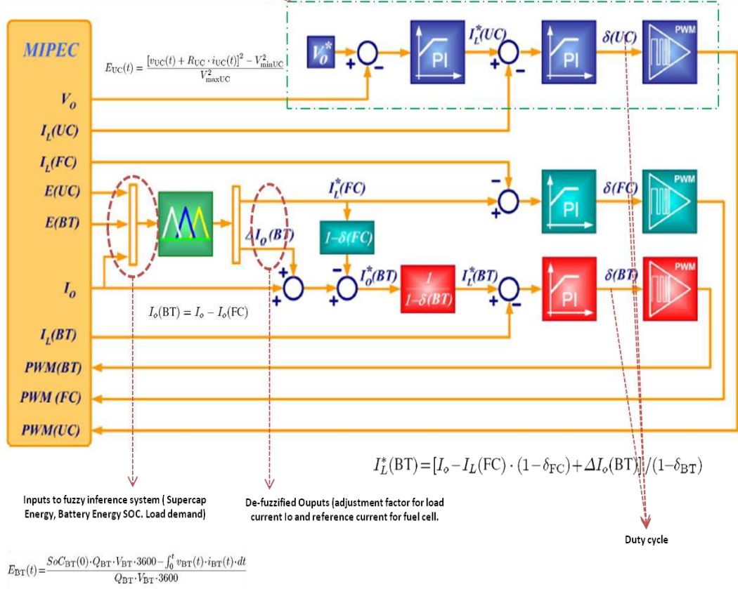
Fig. 25: Block diagram of Fuzzy Logic Supervisory Controller by A.A Ferreira et al [45]
