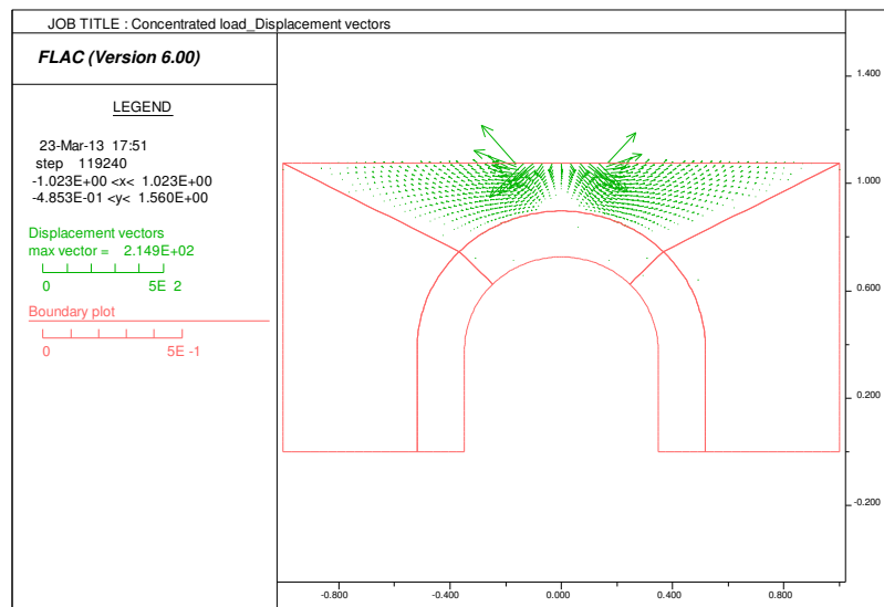
Figure 4.52 Displacement vectors of FLAC model C (1:2:9) under concentrated load
