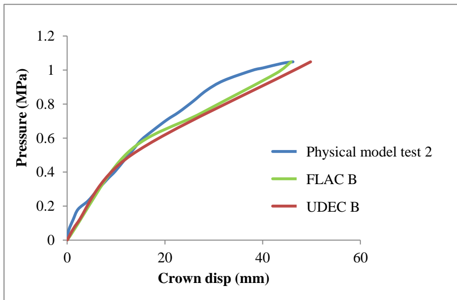
Figure 4.72 Physical model test 2 vs. numerical curves
