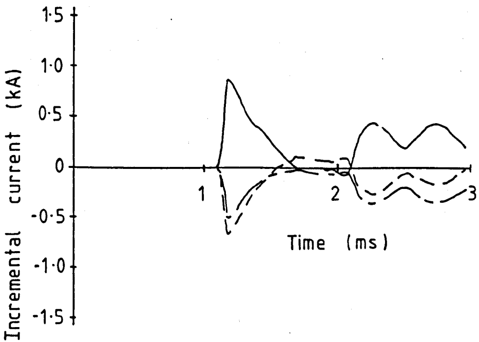
Figure 4.6 Incremental voltage and current transients produced during an external symmetrical fault 340 km from the relaying point (140 km from the far busbar). The fault resistance on each phase was 10 ohms to ground and the fault occurred at phase-a voltage maximum.
