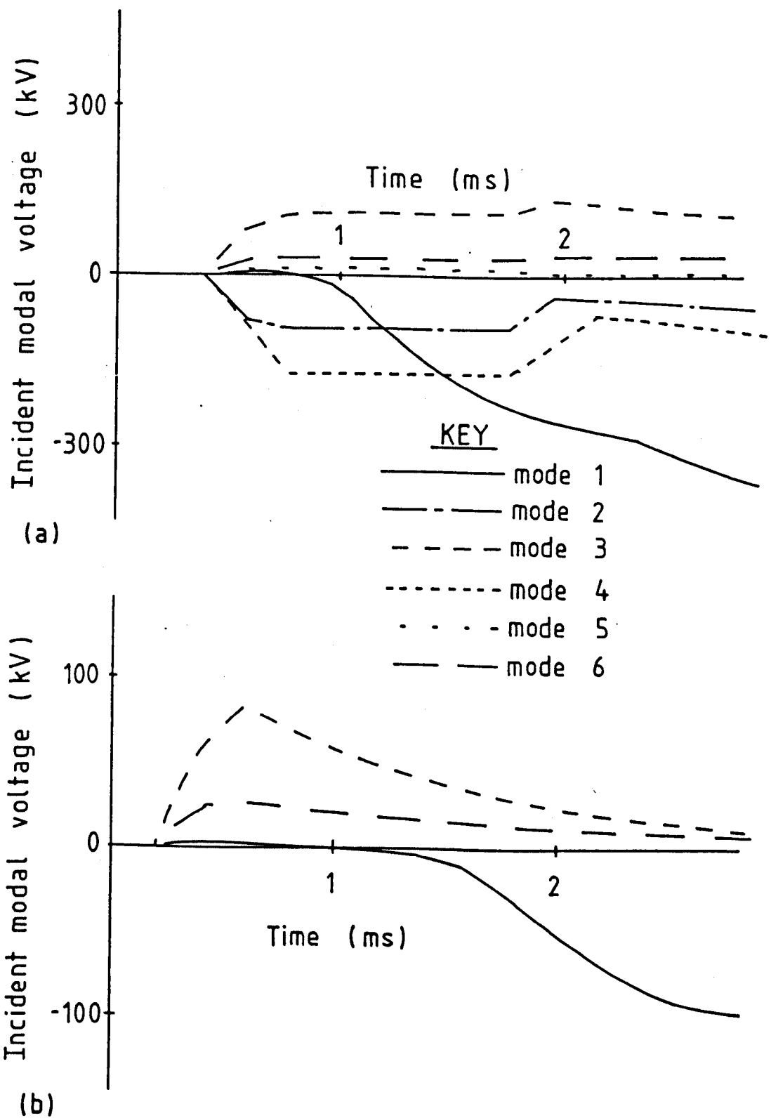
Figure 5.16 The incident modal transients for phase-a to ground faults on a double circuit line with each circuit connected in parallel. (a) An internal fault located 160 km from the relaying point. (b) An external fault located 360 km from the relaying point (160 km from the far busbar).
