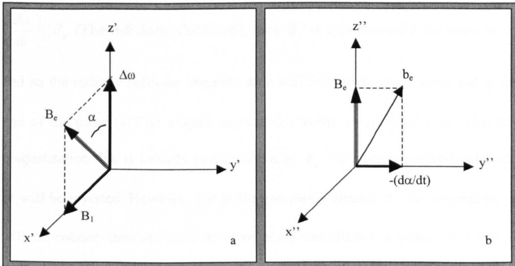
Figure 7.6a – Hyperbolic Secant Pulse in Frame of Reference Rotating at the Instantaneous Frequency of the Pulse. Figure 7.6b – Hyperbolic Secant Pulse in Frame of Reference Where the Direction of the Effect Field, B_e , is Constant Throughout the Pulse.
