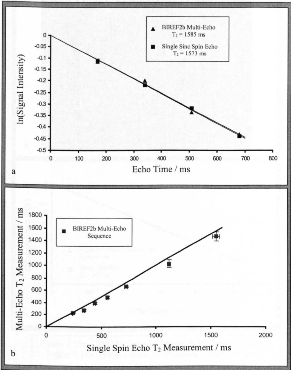
Figure 7.14a – Echo Chain for 0.2 mM CuSO 4 Solution Figure 7.14b – Validation Plot for All Concentrations
