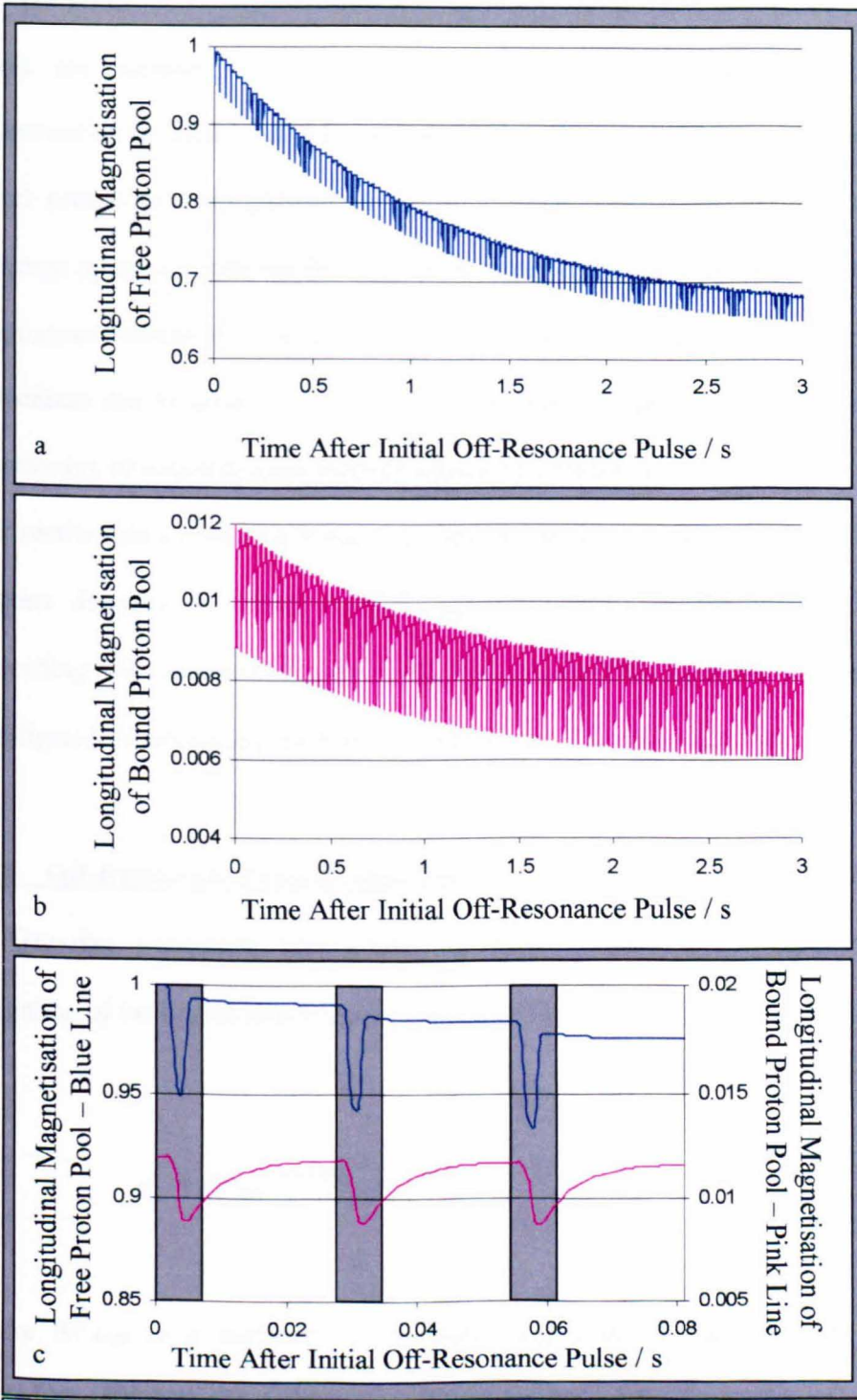
Figure 8.2a – Variation of Free Proton Pool Magnetisation with Time.
