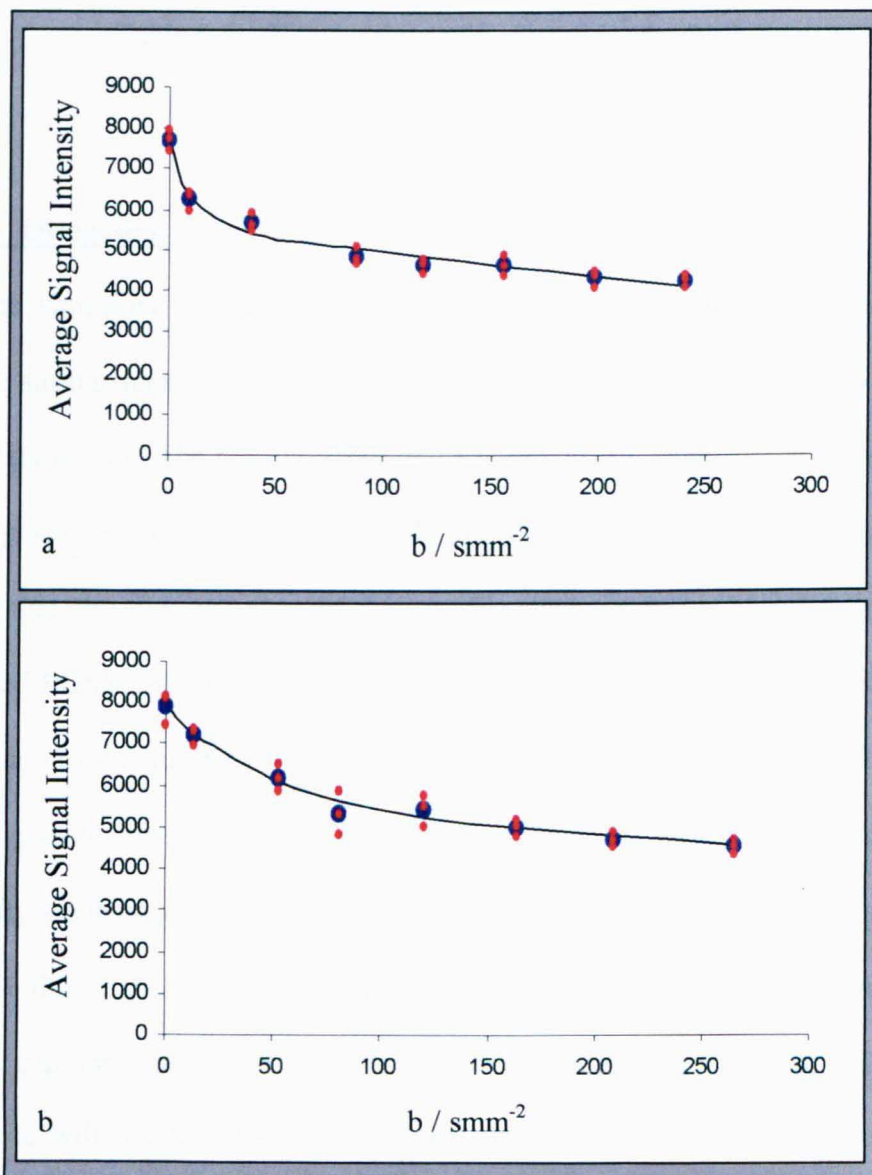
Figure 9.8a – Variation in Average Signal Intensity with Sensitising Gradient Strength for PGSE Sequence. Figure 9.8b – Variation in Average Signal Intensity with Sensitising Gradient Strength for Bi-Polar PGSE Sequence
