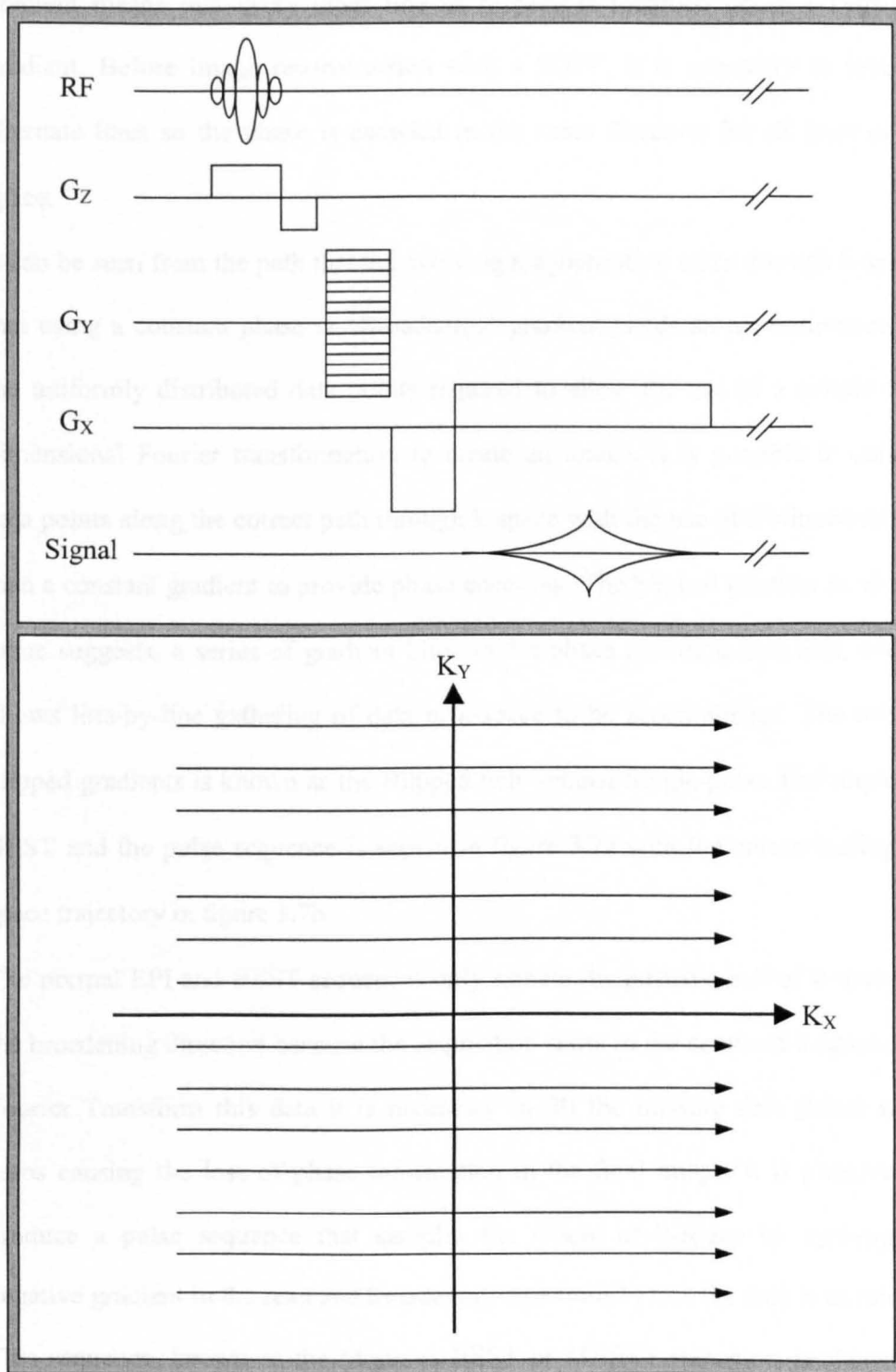
Figure 3.5a – Spin Warp Pulse Sequence Figure 3.5b – Spin Warp k-Space Trajectory
