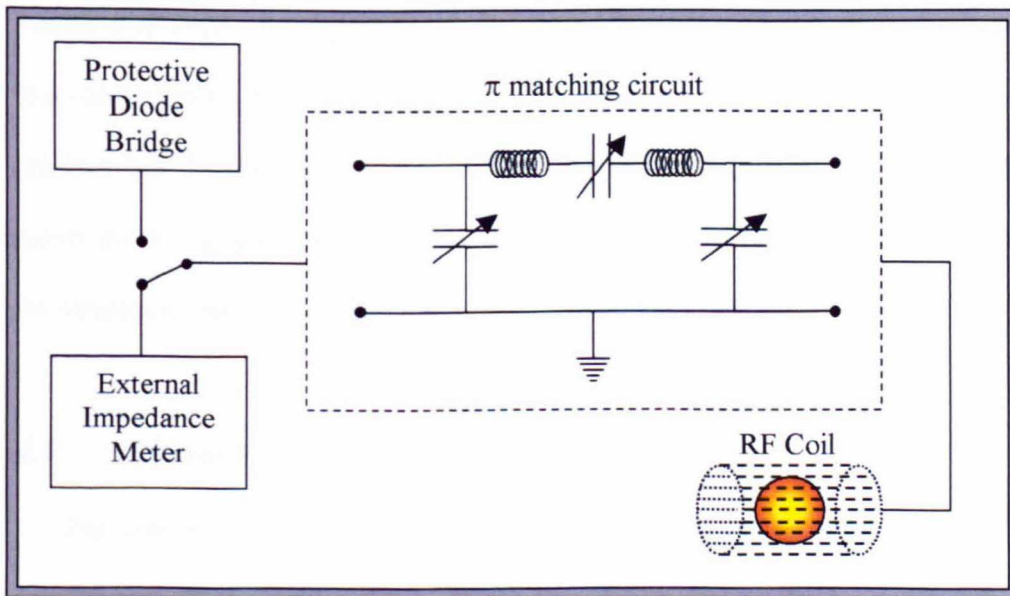
Figure 4.3 – \pi Matching Circuit to Allow for Tuning and Matching
