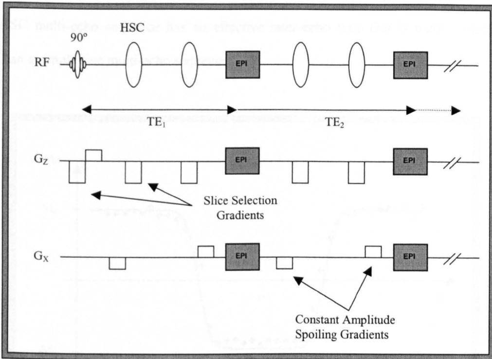
Figure 7.7 – Hyperbolic Secant Multi-Echo Sequence
