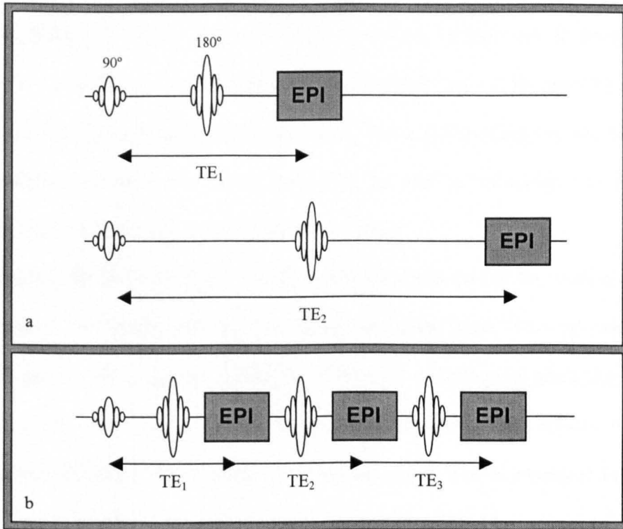
Figure 7.1a – Single Spin Echo EPI Sequence Figure 7.1b – Multi-Echo EPI Sequence
