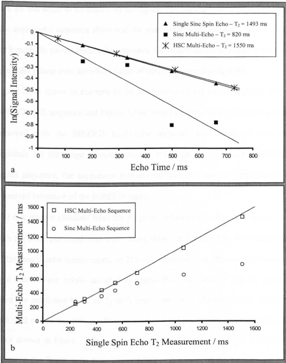
Figure 7.13a – Echo Chains for 0.2 mM CuSO 4 Solution Figure 7.13b – Validation Plot for All Concentrations
