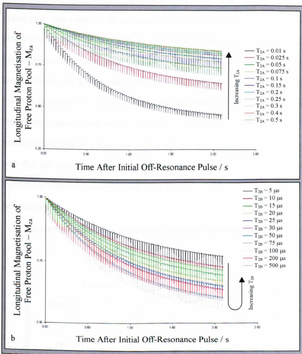
Figure 8.5a – Variation of Free Proton Pool Magnetisation with Time After Initial Off-Resonance Pulse for a Range of Free Proton Pool Transverse Relaxation Times. Figure 8.5b – Variation of Free Proton Pool Magnetisation with Time After Initial Off-Resonance Pulse for a Range of Bound Proton Pool Transverse Relaxation Times.
