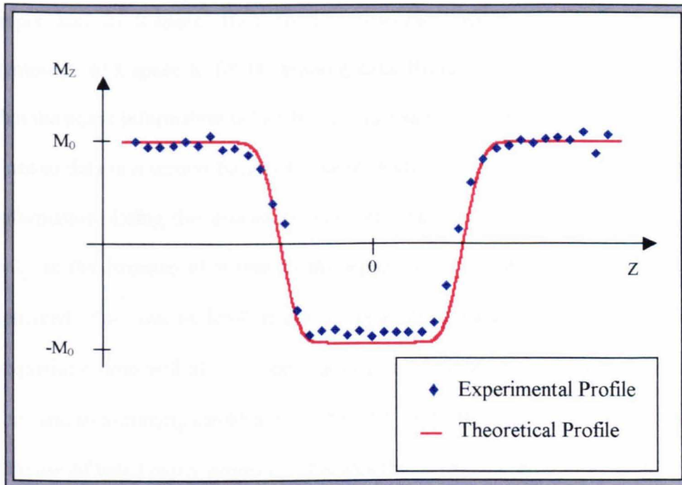
Figure 7.8 – Slice Profile of Hyperbolic Secant Pulse
