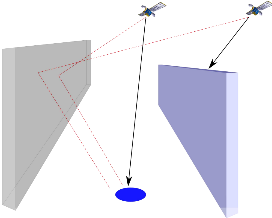
Figure D.1 – Multipath model used in simulator
