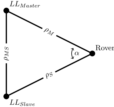
Figure 4.6 – TimeLoc effect on single differencing ( \Delta )
