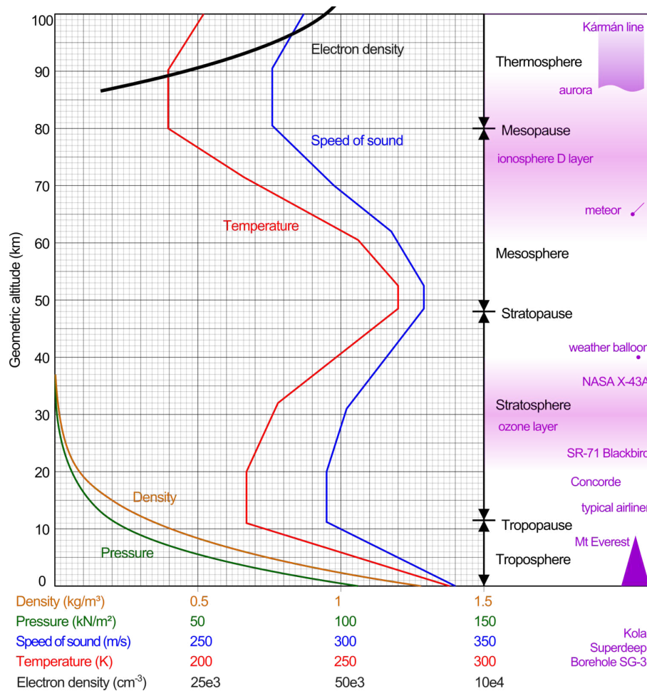
Figure 4.9 – Atmosphere overview
