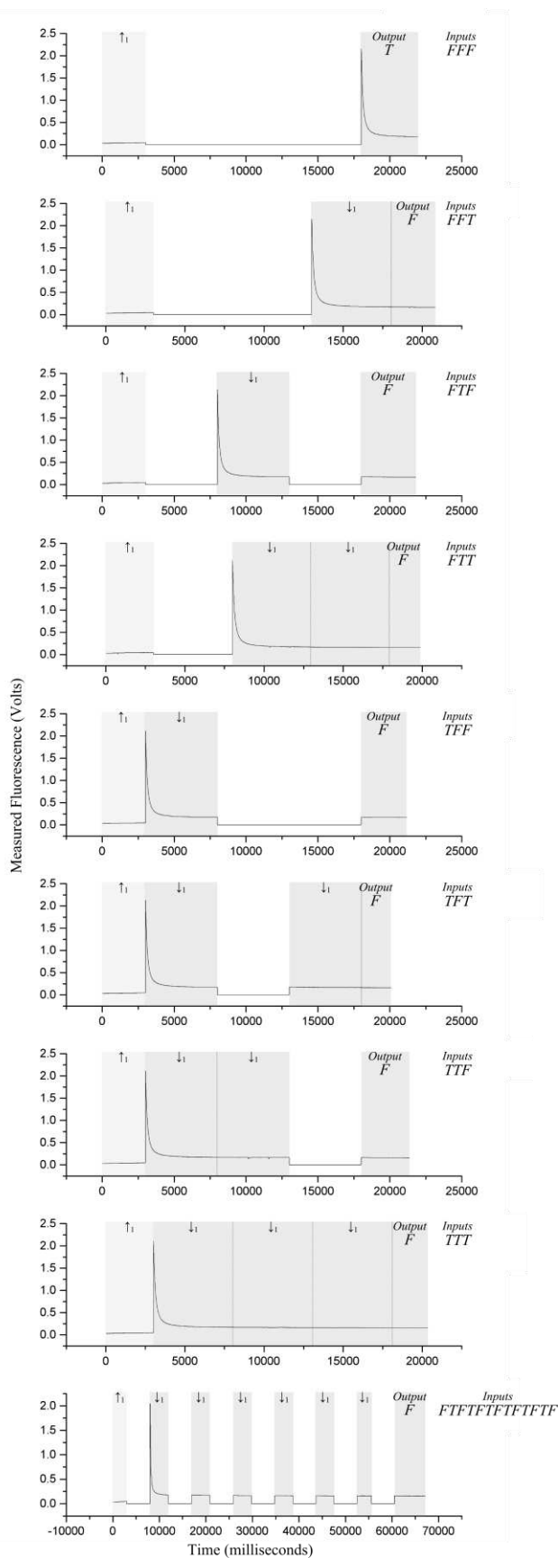
Figure 7.8: Experimentally recorded traces from our system showing nine examples of an n-NOR gate.
