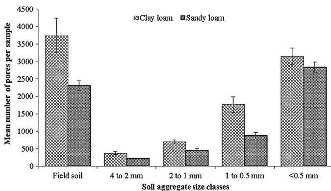
Fig. 6. Mean number of pores per sample for the different aggregate size classes in clay loam and sandy loam soils as measured by X-ray Computed Tomography (texture: F_{1,30} = 22.63, P < 0.001 ; aggregates: F_{1,30} = 84.77, P < 0.001 ; texture \times aggregates: F_{1,30} = 3.71, P < 0.05 ). Mean values are shown, error bars indicate standard error of mean, n = 4 .
