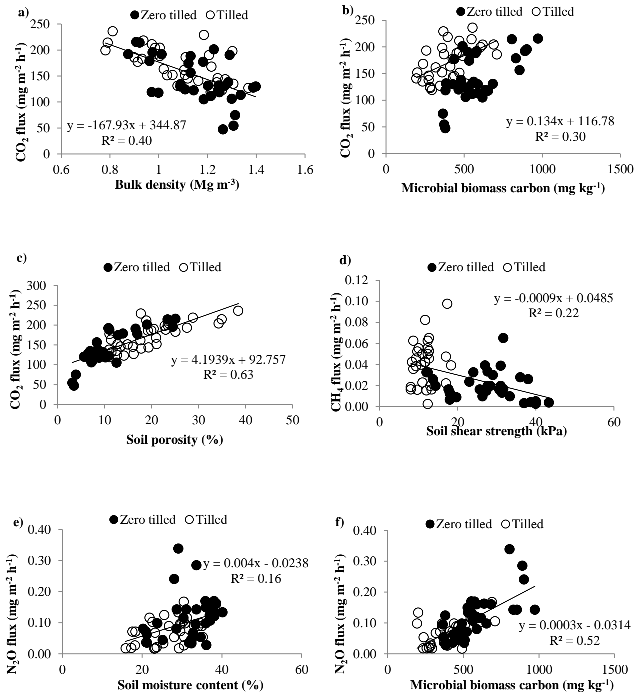
Fig. 4.11. Illustration of important relationships between soil bio-physical properties and GHG release. (a) soil bulk density and CO 2 flux from soil; F_{1,64} = 42.08 , P < 0.001 (b) microbial biomass carbon and CO 2 flux; F_{1,64} = 5.89 , P < 0.05 (c) soil porosity and CO 2 flux; F_{1,64} = 110.14 , P < 0.001 (d) soil shear strength and CH 4 flux; F_{1,64} = 14.08 , P < 0.001 (e) soil moisture content and N 2 O flux, ; F_{1,64} = 12.62 , P < 0.001 and (f) microbial biomass carbon and N 2 O flux; ; F_{1,64} = 69.5 , P < 0.001 .
