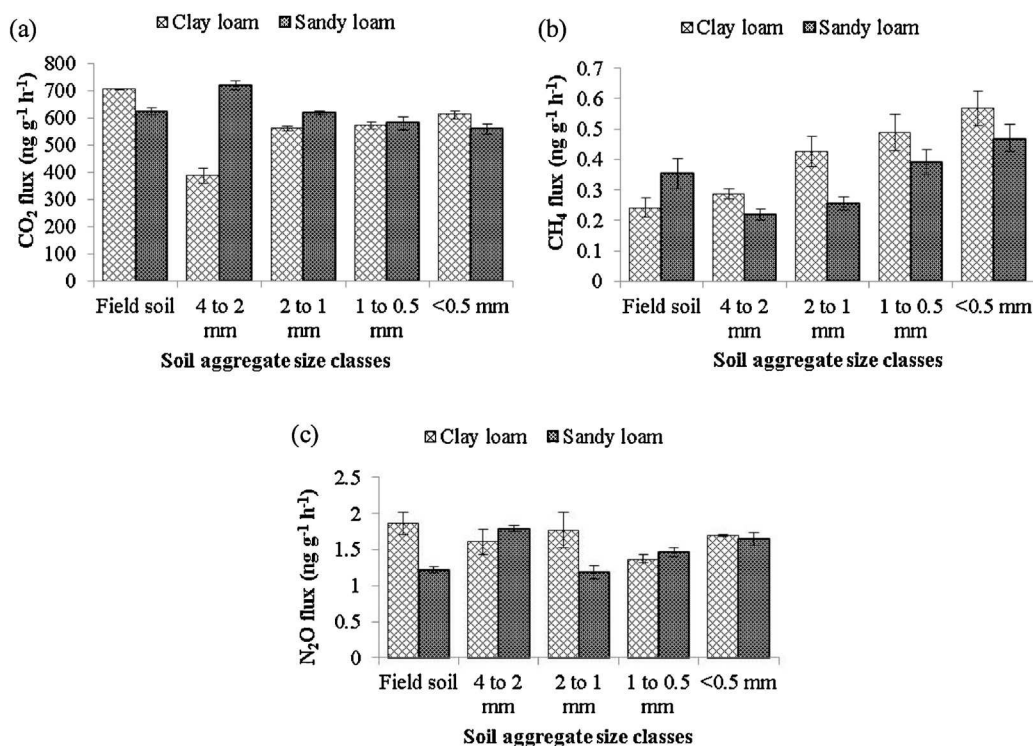
Fig. 4. Differences in average fluxes of \text{CO}_2 , \text{CH}_4 and \text{N}_2\text{O} ( \text{ng g}^{-1} oven dried soil \text{h}^{-1} ) in different aggregate size fractions in clay loam and sandy loam soils (a) \text{CO}_2 flux: texture: F_{1,30} = 26.59 , P < 0.001 ; aggregates: F_{1,30} = 13.30 , P < 0.001 ; texture \times aggregates: F_{1,30} = 51.43 , P < 0.001 ; (b) \text{CH}_4 flux: texture: F_{1,30} = 5.93 , P < 0.05 ; aggregates: F_{1,30} = 13.39 , P < 0.001 ; texture \times aggregates: F_{1,30} = 3.21 , P < 0.05 ; (c) \text{N}_2\text{O} flux: texture: F_{1,30} = 6.97 , P < 0.05 ; aggregates: F_{1,30} = 2.03 , NS; texture \times aggregates: F_{1,30} = 5.18 , P < 0.01 ; Mean values are shown, error bars indicate standard error of mean, n = 4 .
