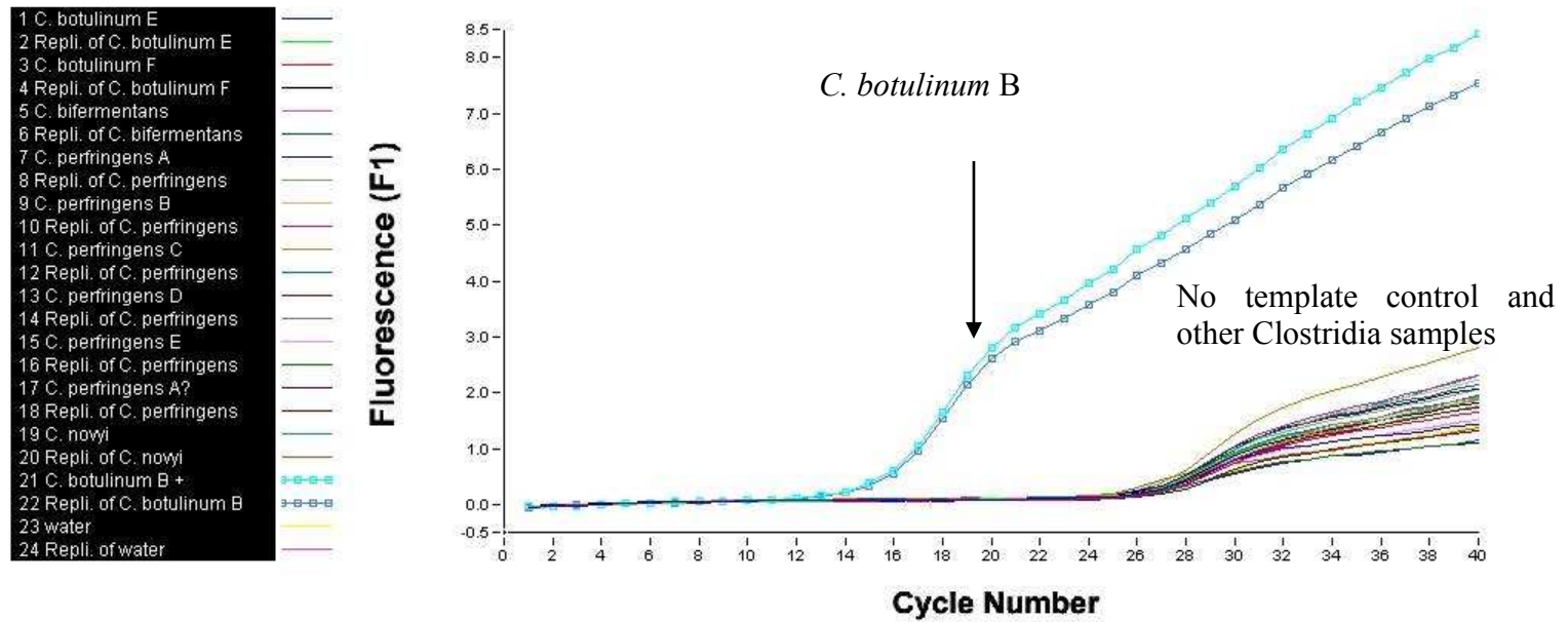
Figure 3.5 Dependence of relative fluorescence on PCR cycle number for C. botulinum B sybr Green I PCR assay containing the bont B1 primers, in the presence of various Clostridial DNAs.
