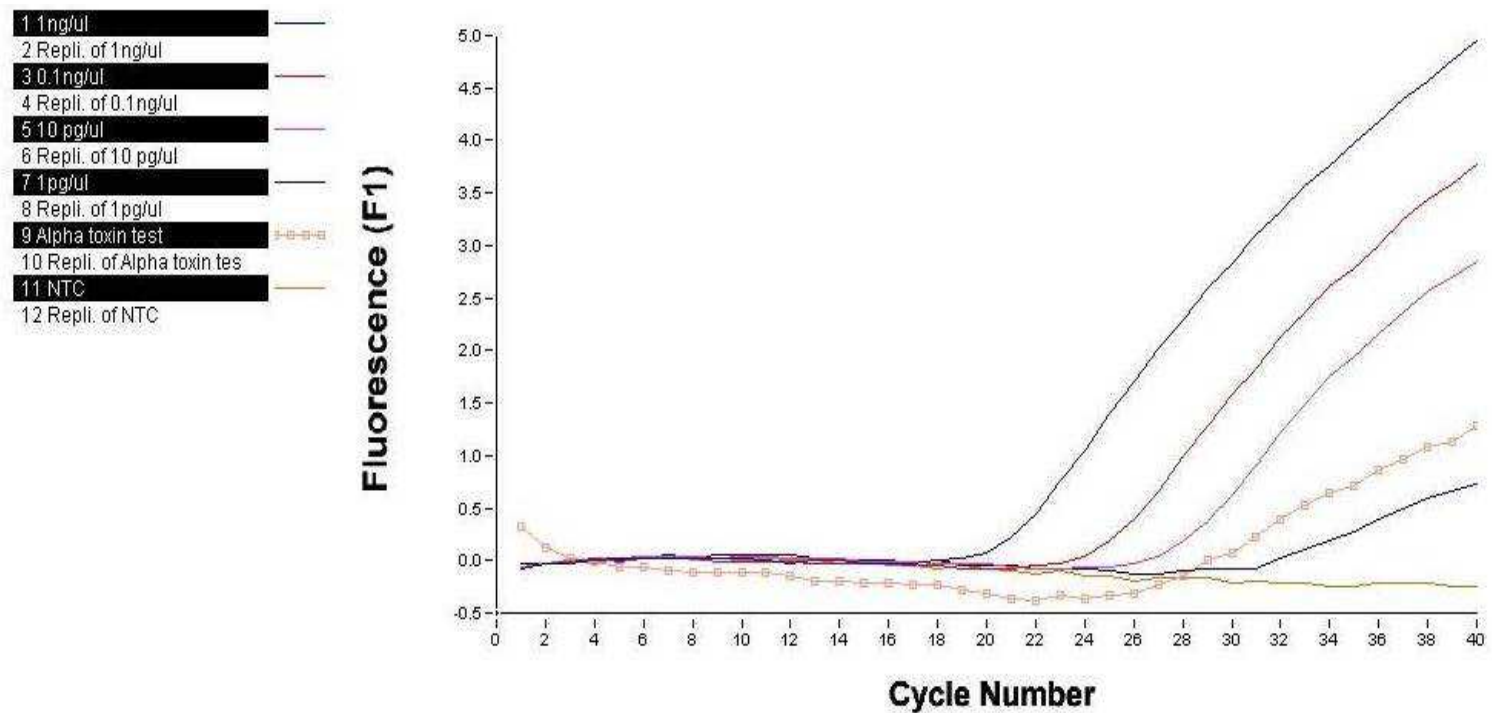
Figure 3.22. Quantitative PCR analysis of purified alpha toxin with the plc primer and probe set. DNA standards are shown in unbroken lines, the alpha toxin sample is shown in the hatched line. Samples were run in duplicate, however only single samples are shown for illustrative purposes.
