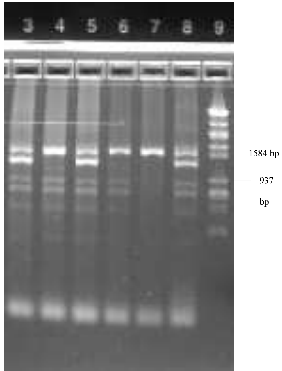
Figure 5.9. RFLP analysis of a 1.6 kb fragment of the preproricin gene of R. communis cultivars. The DNA was cut with EcoRI and HindIII and resolved on a 2 % agarose E-gel for 30 minutes. Lane 3, Shang Dong 108; Lane 4, Jin Castor 2; Lane 5, Sanguinis; Lane 6, Zanzibar; Lane 7, Zibimas; Lane 8, Zibo 1; Lane 9, Molecular weight marker III (Roche).
