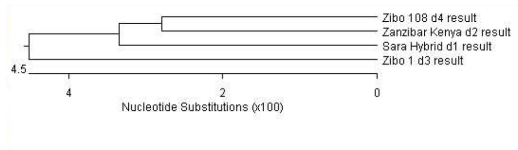
Figure 5.5. Biotage generated sequence alignment and dendrogram for four cultivars of R. communis .
