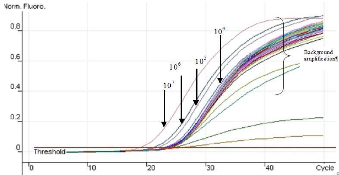
Figure 4.18 - Detection limit of B. cereus immuno-phage PCR. Immuno-phage PCR was carried out using a range of B. cereus spore concentrations from 10^7 to 10^0 / ml. Phage concentration ranged from 10^7 transforming units (TU)/ml to 10^5 TU/ml. Positive amplification was observed using 10^7 tu/ml only; using diluted phage resulted in background amplification.
