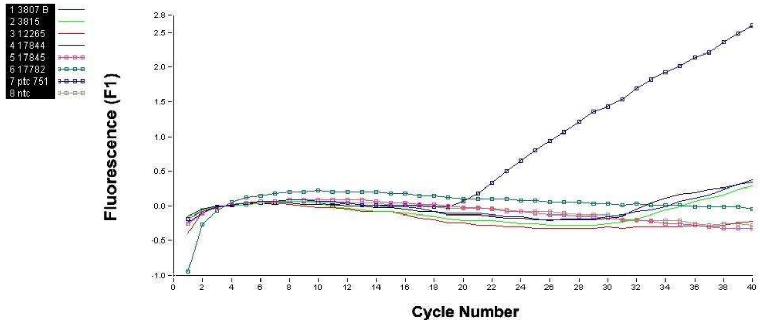
Figure 3.8 Analysis of C. botulinum B DNA using the bont B PCR primer and probe set. An increase in fluorescence was seen with DNA obtained from strain 751 (positive template control). A weak increase in fluorescence was also seen with strains 3807, 3815 and 17844. No increase in fluorescence was observed with strains 17845 and 17782,
