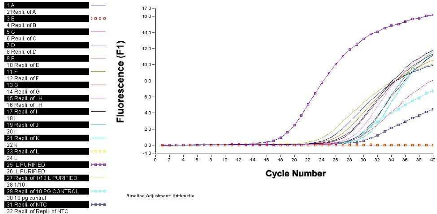
Figure 3.18. Analysis of samples taken throughout the 12 stage recombinant V antigen purification process using the Y. pestis rV PCR assay designed for this study. An increase in fluorescence was observed in all of the above samples apart from the no template control (NTC, samples 31 and 32). rV antigen was extracted by sonication and purified using a GST affinity column (A-D), protease cleaved (1-5, samples E-K respectively) and pooled. The pooled product was processed using a QIAamp DNA mini kit.
