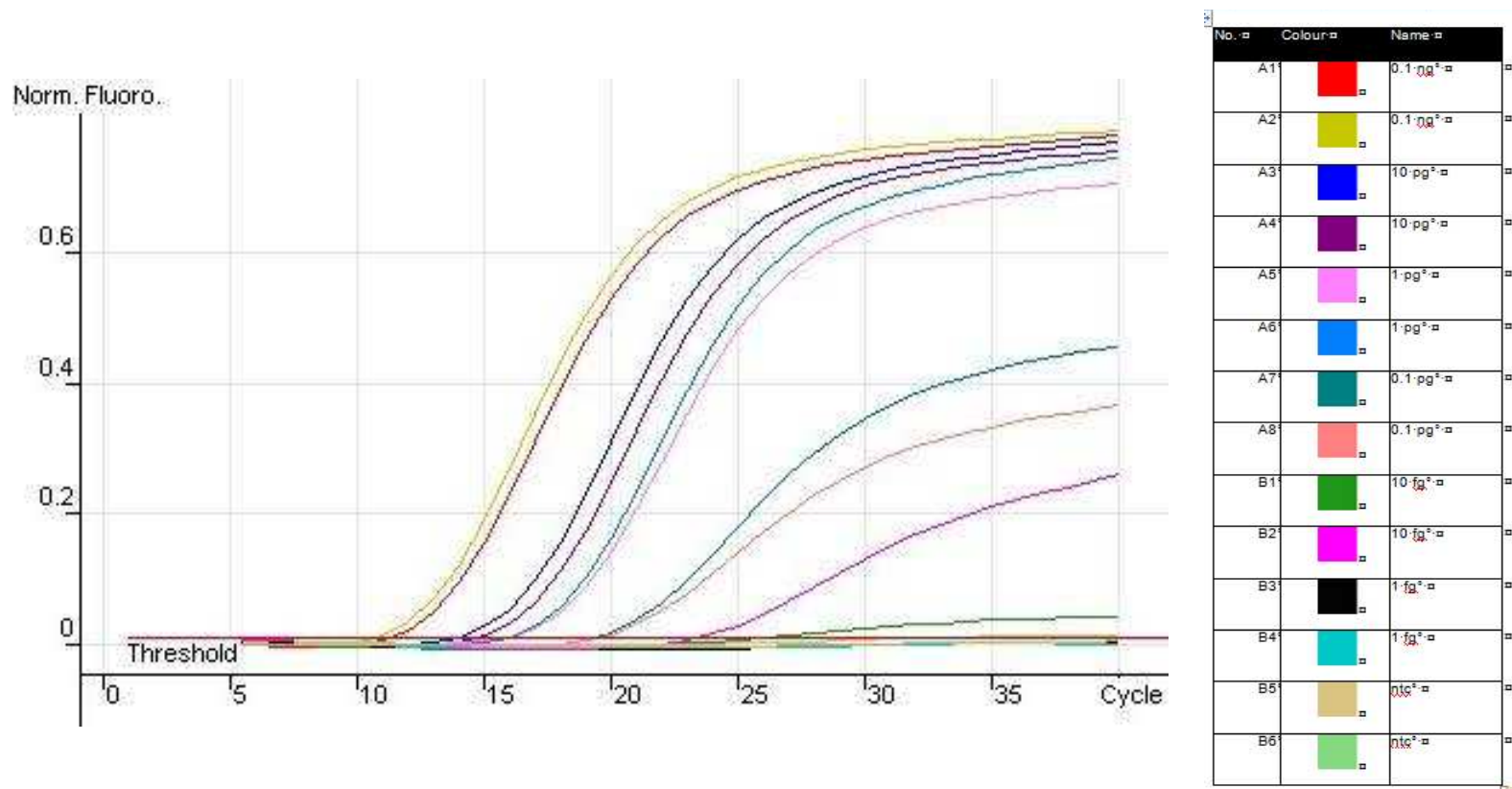
Figure 3.24 Detection limit of un-optimised C. botulinum A DNA in a multiplexed A/B PCR assay. DNA standards were prepared from C. botulinum A NCTC 2916 and amplified with the bont A/B multiplex using 500nm of each type A primer. An increase in fluorescence was observed with DNA concentrations between 0.1 ng/ \mu l and 10fg/ \mu l
