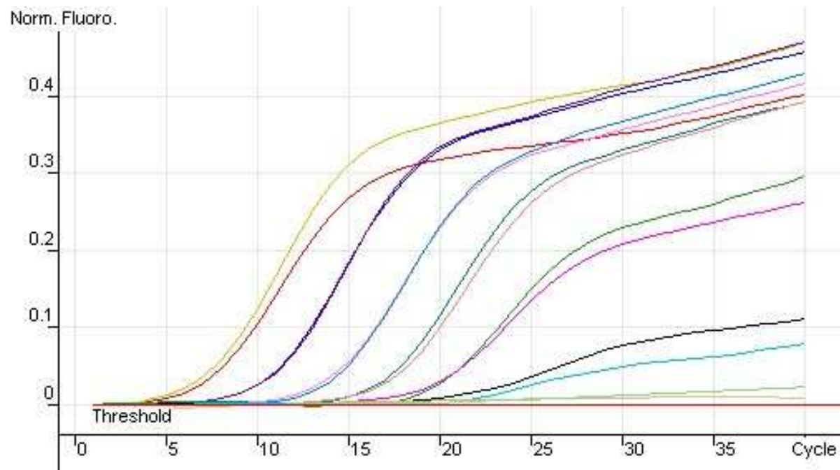
Figure 3.26 Detection limit of C. botulinum A DNA in an optimised multiplexed A/B PCR assay. DNA standards were prepared from C. botulinum A NCTC 2916 and amplified with the bont A/B multiplex using 50nm of each type A primer, with increased amounts of Taq polymerase, dNTPs and MgCl 2 . An increase in fluorescence was observed with DNA concentrations between 0.1 ng/ \mu l and 10fg/ \mu l.
