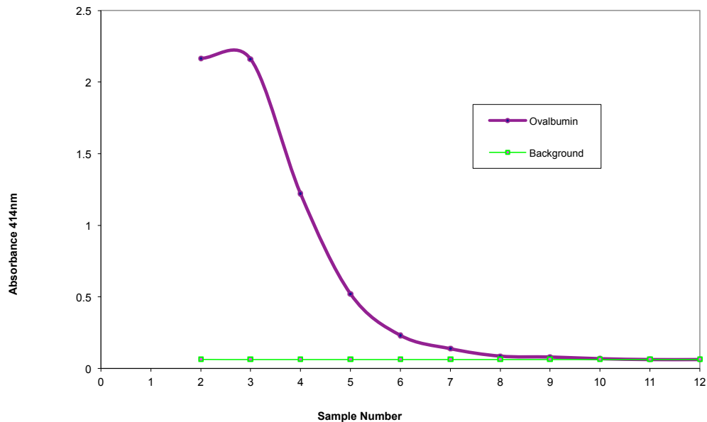
Figure 4.2b. Example ELISA A 414 nm results for ovalbumin concentrations diluted 3-fold, starting at 1000 ng/ml. The primary antibody was bound to the surface of the ELISA plate. Ovalbumin was subsequently allowed to bind to the antibody. A secondary biotin-labelled antibody was bound to the immobilised ovalbumin. Streptavidin labelled with horseradish peroxidase (HRP) was bound to the sandwich. This was followed by the addition of the HRP substrate hydrogen peroxide plus ABTS resulting in a colorimetric change which can be measured at A 414 nm and plotted on a graph. The background fluorescence was 0.062.
