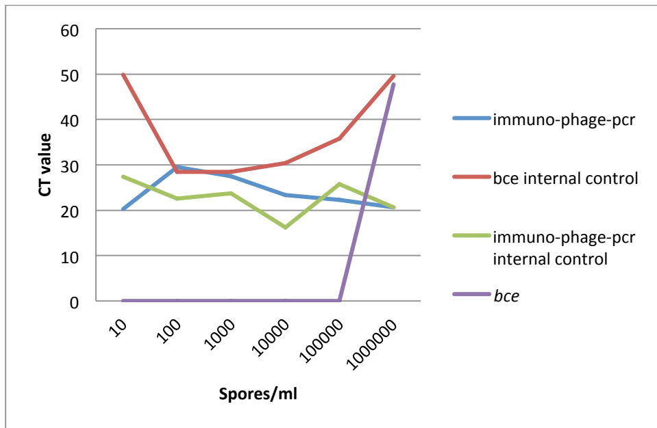
Figure 4.21. Summary of cycle threshold values obtained from immuno-phage-PCR detection of Bacillus cereus spores. Detection of bce and scFv genes, plus their respective internal controls, was carried out using real time PCR.
