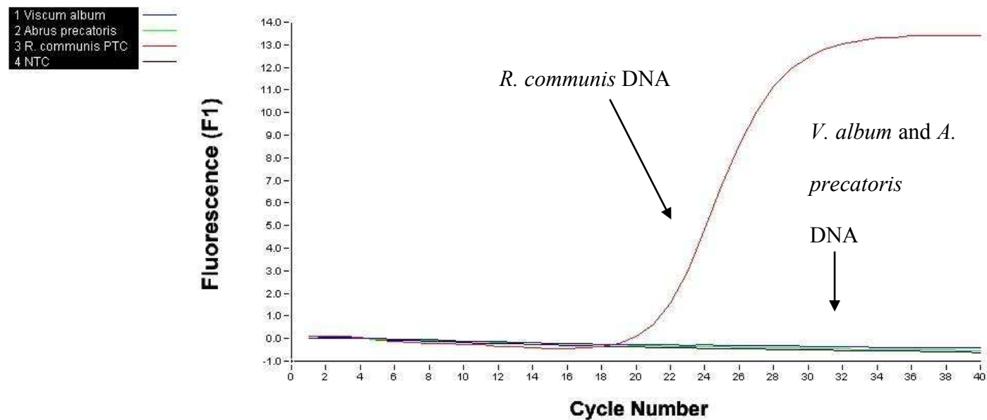
Figure 3.19 Real-time PCR analysis of DNA extracted from the ribosome inactivating protein producing plants R. communis , V. album and A. precatoris , using ricin specific PCR primers and probes. An increase in fluorescence was observed with the R. communis sample.
