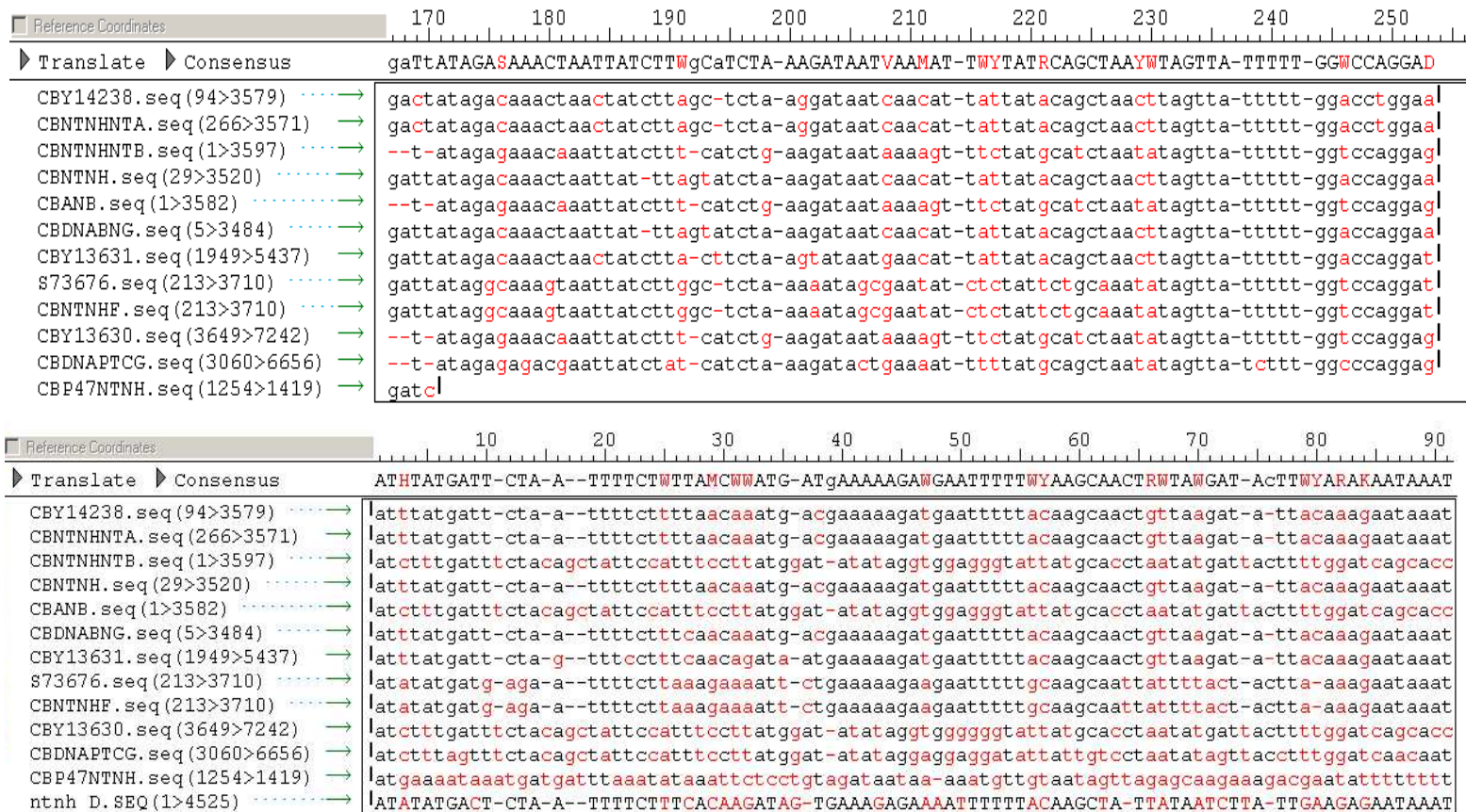
Figure 3.1 Alignment data used to design PCR primers for the detection of Clostridium botulinum ntnh gene. DNA sequences from the ntnh gene of various strains were obtained from Genbank and aligned in SeqMan (DNASTAR, Lasergene 6). The resulting consensus sequence was exported into Primer Express v 1.0 (Applied Biosystems) for primer design. The ntnh amplicon designed for this study is shown. The ntnh F primer used was CTCCTGGACCAAAAATAAC (position 253-232 of the top alignment). The reverse primer sequence was ATCTTTCATTCTACAGCTATTC (position 1-24).
