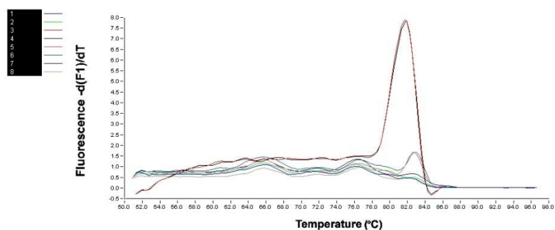
Figure 1.5 Example melt curve analysis graph. The apex of the curve represents the point at which an amplicon ‘melts’ and becomes single stranded, leading to a rapid loss of fluorescence. This melting temperature (T m ) can be used to differentiate between PCR products.
