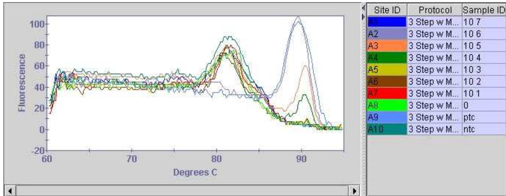
Figure 4.19 - Melt curve analysis of scFv PCR products PCR of I- \phi -PCR samples containing 10^7 to 10^3 spores/ml produced a specific product with a T_m of 90^\circ\text{C} . Non specific products were also observed, with a T_m of 81^\circ\text{C} .
