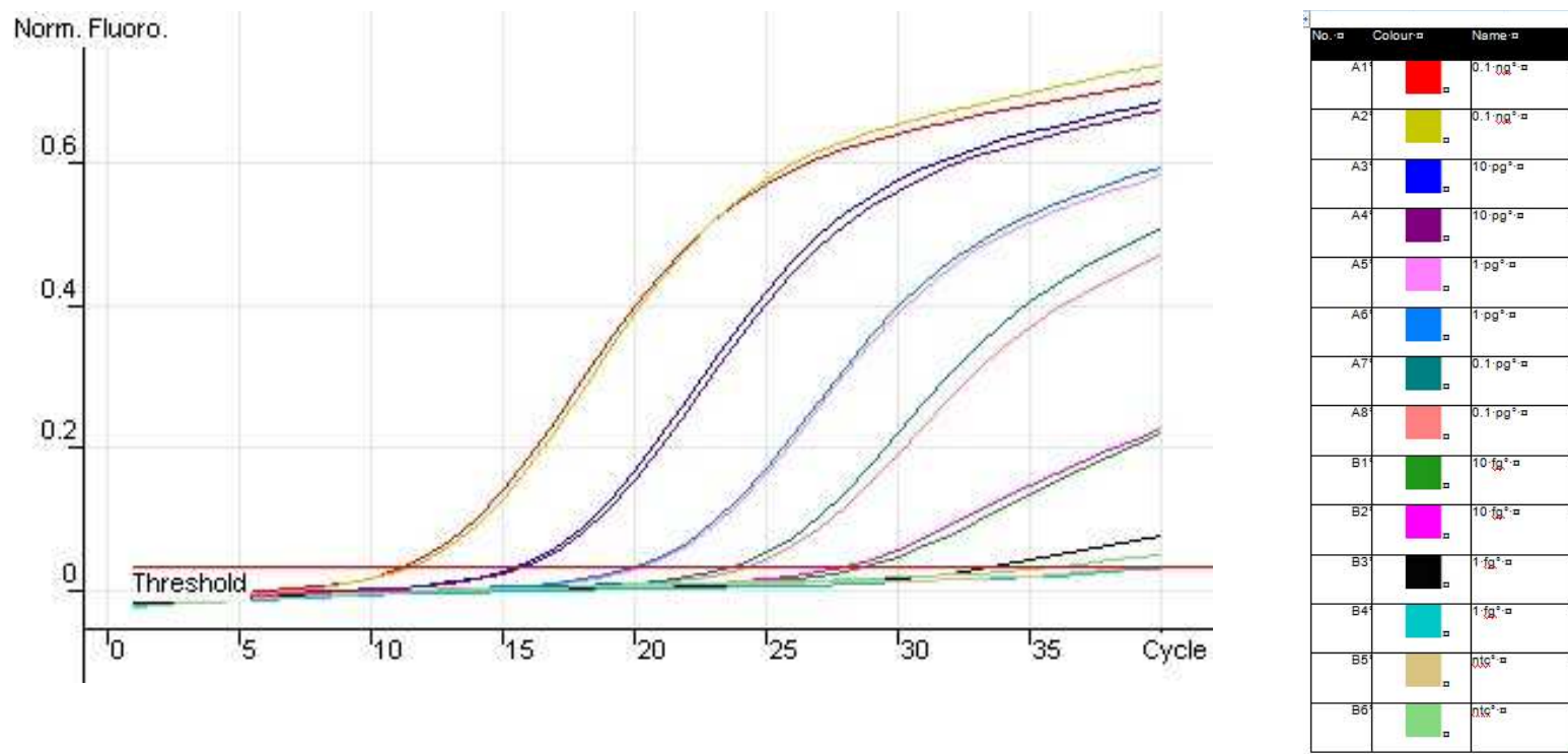
Figure 3.27. Detection limit of C. botulinum B DNA in an optimised multiplexed A/B PCR assay. DNA standards were prepared from C. botulinum B ATCC 17841 and amplified with the bont A/B multiplex using 500nm of each type B primer with 50 nM of type A primer. Extra Taq polymerase, dNTPs and MgCl 2 were also added to the multiplex assay. An increase in fluorescence was observed with DNA concentrations between 0.1 ng/ \mu l and 1fg/ \mu l.
