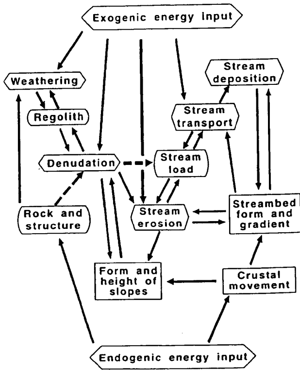
Components and interactions of the fluvial landform system (schematic)
