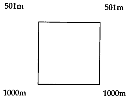
Figure 5.2 Level Trend Service Analysis for Er Rif Area of Morocco
