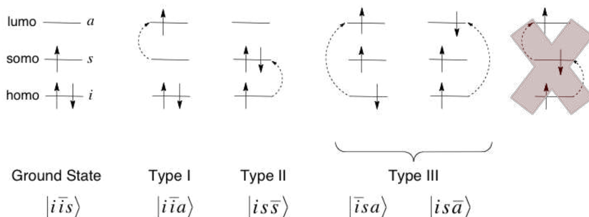
Figure 4.8 The types of excitation arising from a doublet ground state. Where i represents a doubly occupied orbital, s represents the singly occupied orbital, and \alpha represents an unoccupied orbital. The presence or absence of a bar over i , s or \alpha indicates a beta or alpha spin electron, respectively. [131]
