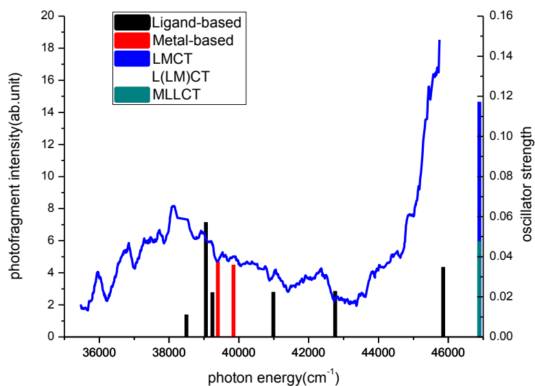
Figure 6.6 UV photofragmentation spectroscopy of [\text{Cu}(\text{benzene})_2]^{2+} overlaid by tabulated TDDFT calculated excitation energies and oscillator strengths using CAM-B3LYP functional, 6-311++G(d,p)/SDD as basis sets, a) Calculated transitions for all optimized structures of \text{C}_2 and \text{C}_{2v} [\text{Cu}(\text{benzene})_2]^{2+} conformers using BVP86, PBE0 and TPSSh, respectively; b) The transitions are sorted in their nature.
