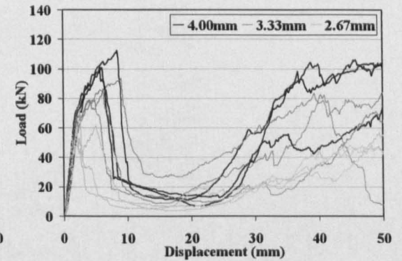
16mm Hole
