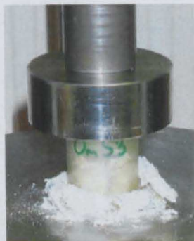
34mm crush
