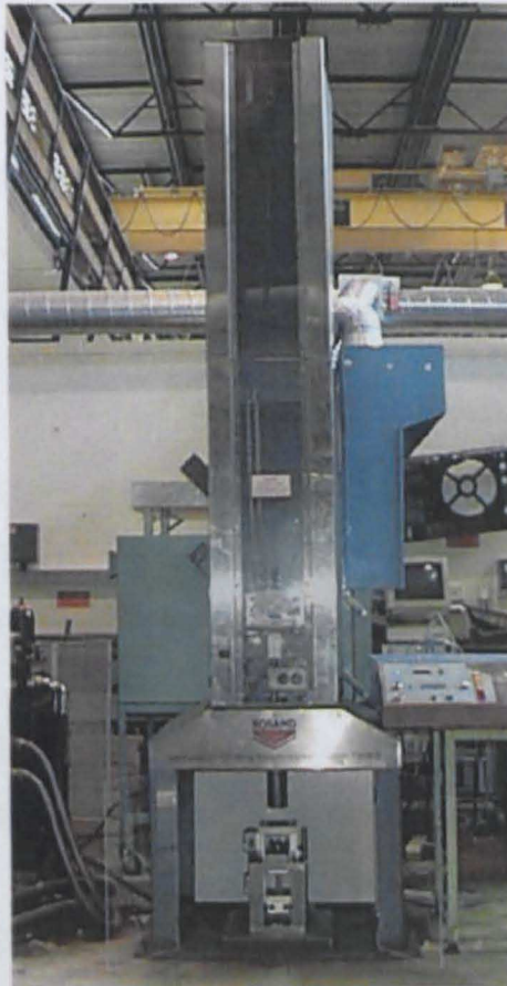
Figure 3-16 - Rosand falling weight impact test machine
