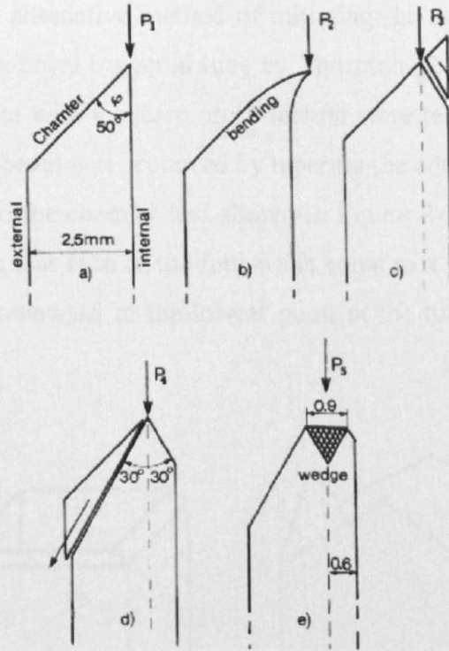
Figure 2-10 - Schematic representation of the initial crushing process for chamfer angles of between 30° and 80° [29]
