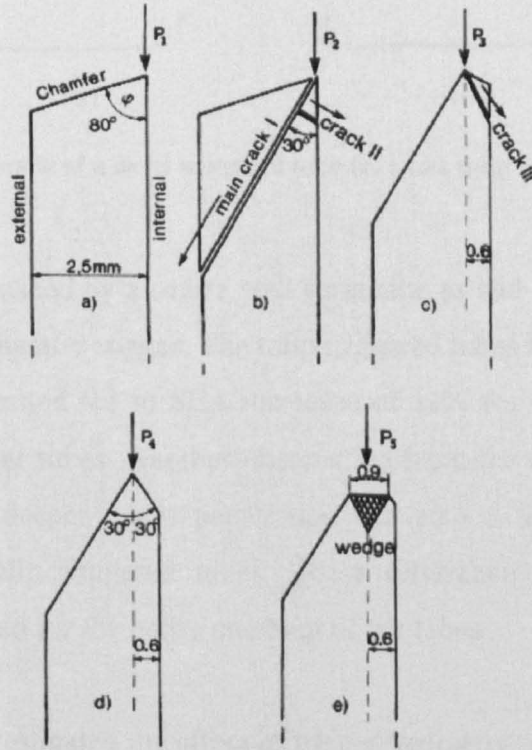
Figure 2-11 – Schematic representation of the initial crushing process for chamfer angles of greater than 80° [29]
