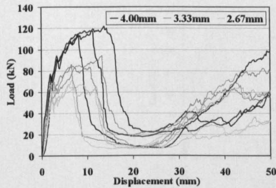
12.5mm Hole
