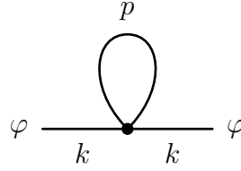
Figure 4.7: The pure scalar bubblegum diagram with a \varphi^4 vertex
