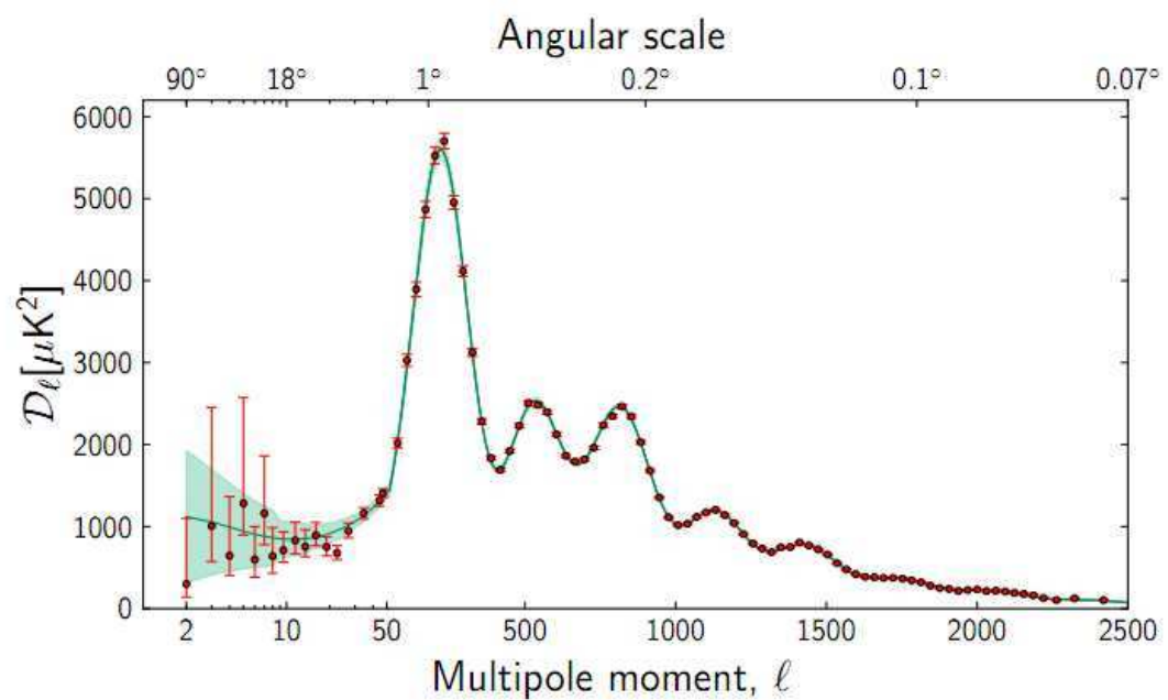
Figure 1.2: The temperature angular power spectrum of the primary CMB from Planck (points) and the prediction from \Lambda CDM (green line). The shaded region represents cosmic variance. (Figure from Planck Collaboration, 2013). \Lambda CDM is in excellent agreement with the observed points.
