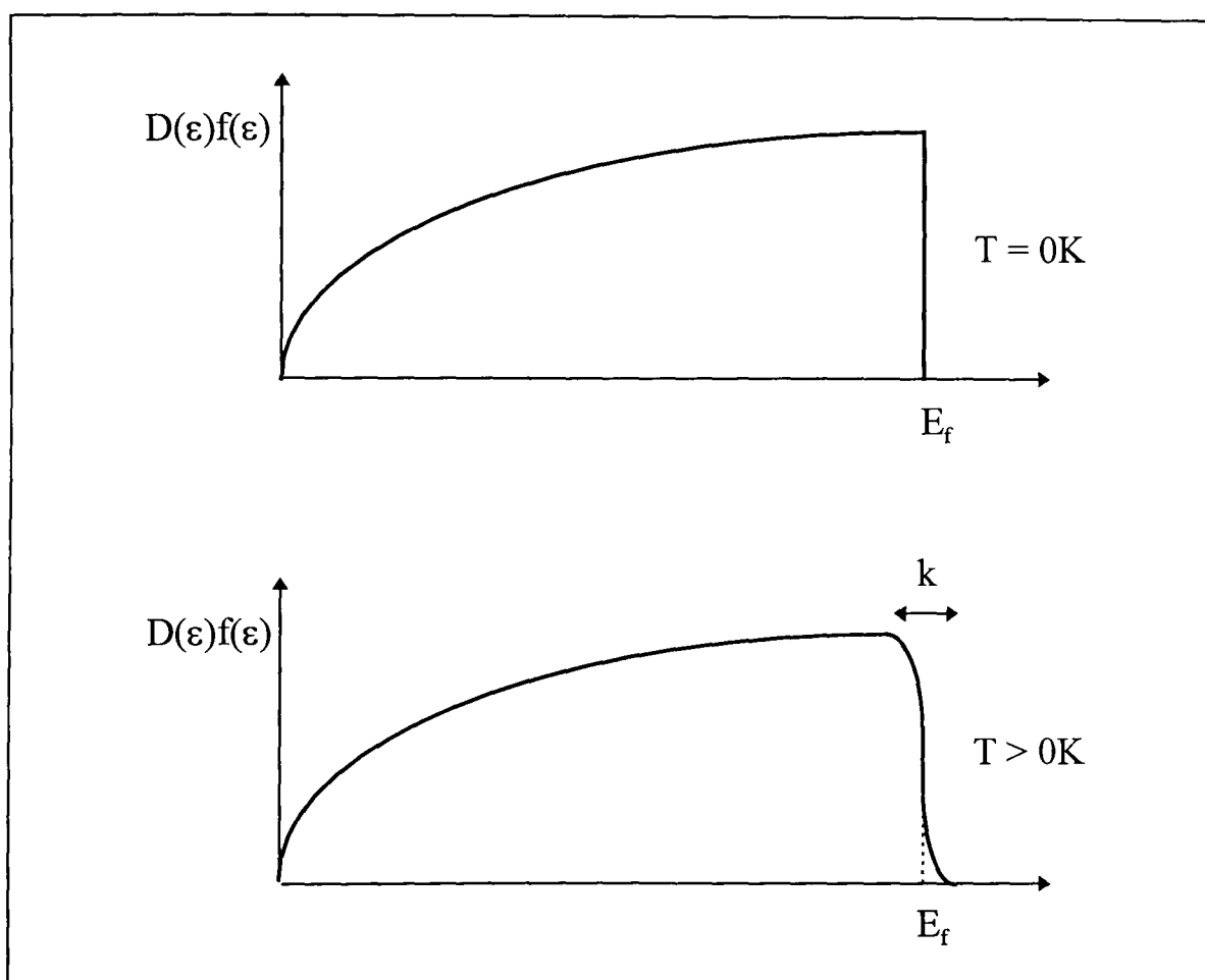
Fig 1.2: Plot of population of states against energy for a 3D free electron gas at T = 0\text{K} and T > 0\text{K} .
