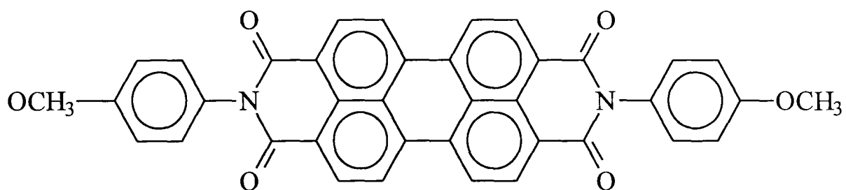
MOPPCI: dimethoxyphenyl perylenetetracarboxylic acid diimide
