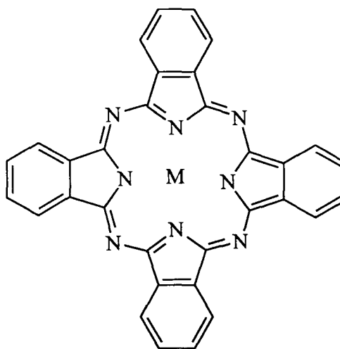
Fig 3.1: Molecular structure of a metal phthalocyanine
