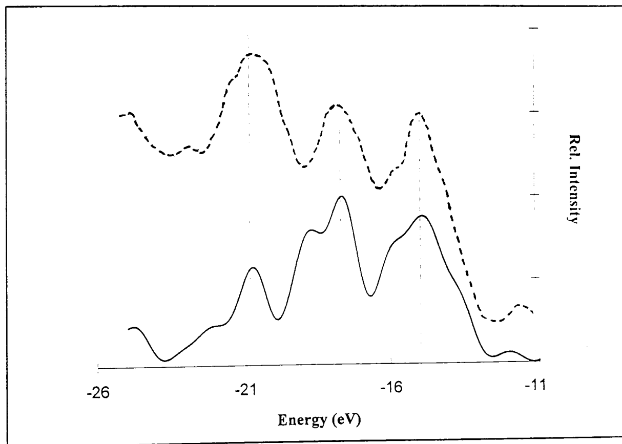
Fig 6.17: Simulated PES for a 1D H 2 Pc stack (solid line). The energy axis is multiplied by 1.25 for the experimental spectrum (ref 152) in the dotted line.
