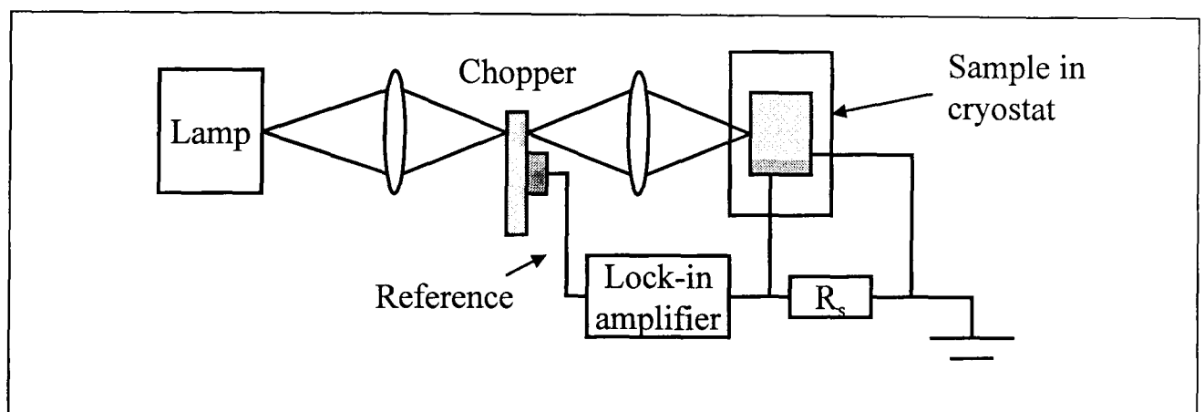
Fig 4.5 Chopped light photoconduction apparatus.
