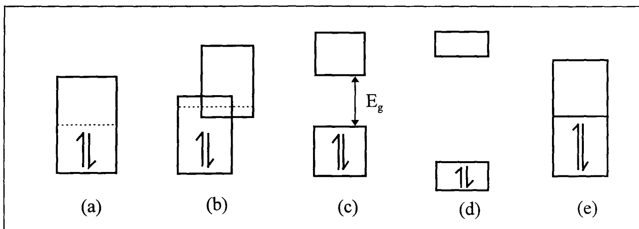
Fig 1.4: Relationship between electrical properties of solids with the location and filling of the energy bands. (a) Metal with a partially filled band. (b) Metal generated by the overlap of filled and empty bands. (c) Semiconductor characterised by a small gap between the filled and empty bands. (d) Insulator with a large gap between the filled and empty bands. (e) Semi-metal where the filled and empty bands just touch from ref. 149.
