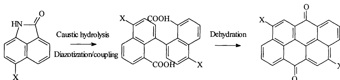
Fig 3.11: Synthetic pathway to 2,7-dihalo-anthanthrones.
