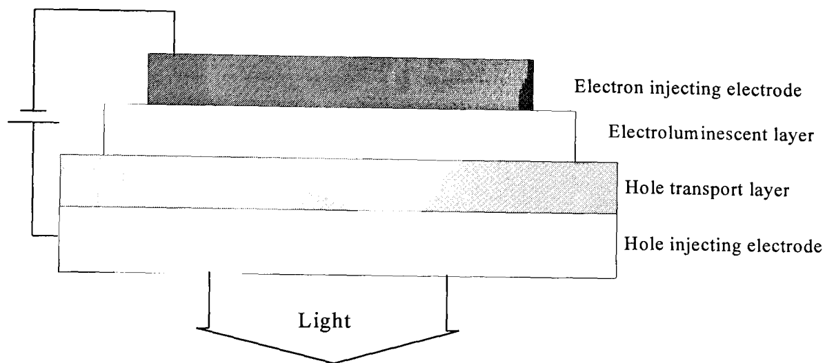
Fig 7.6: Schematic design of a bilayer electroluminescent cell
