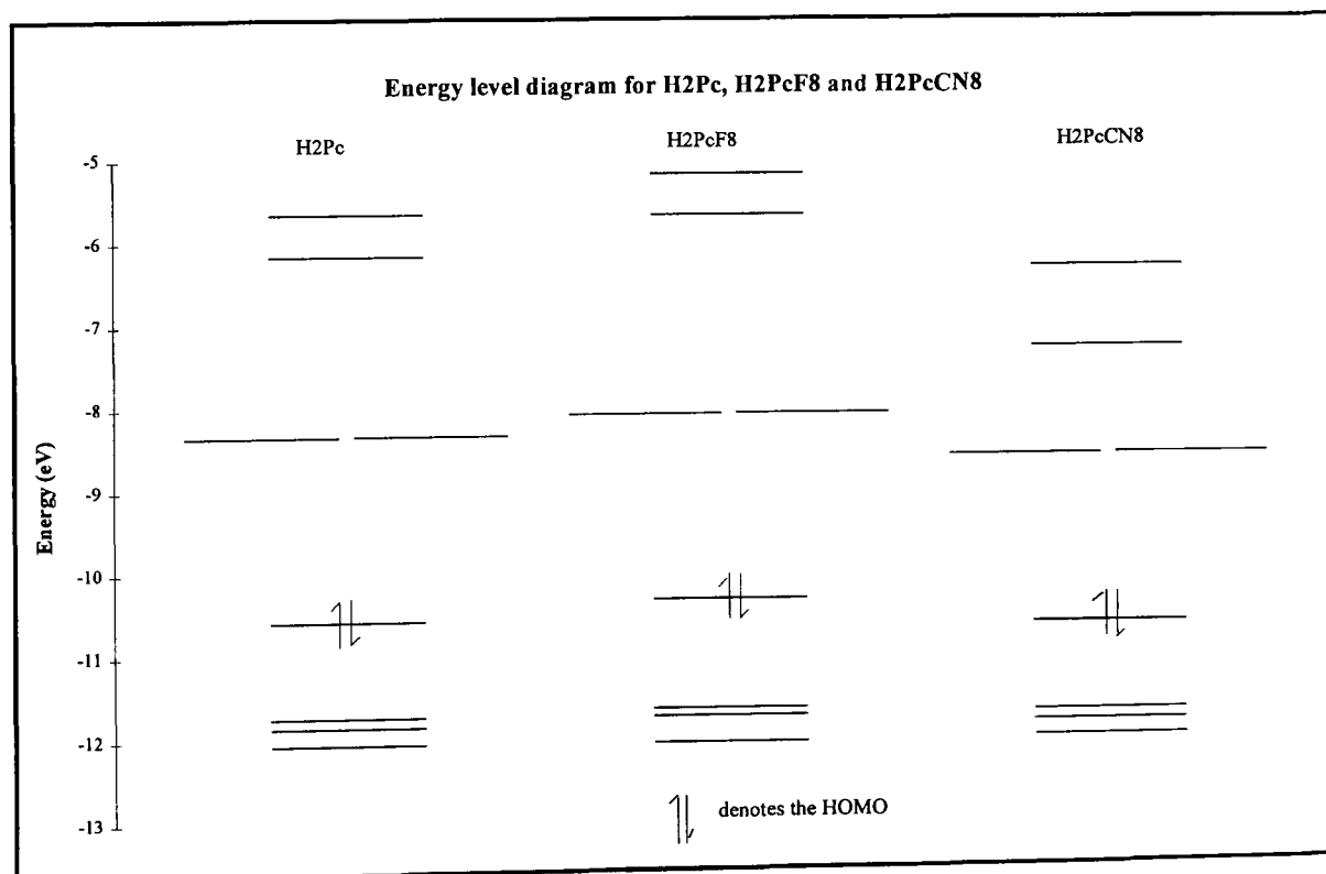
Fig 6.11: Energy level diagram for metal free phthalocyanine, octofluoro metal-free phthalocyanine and octocyno metal-free phthalocyanine calculated using the EH method.
