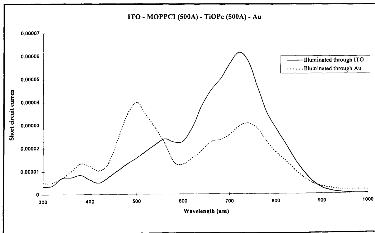
Fig 5.6: Action spectra for ITO - MOPPCI (500Å) - TiOPc (500Å) - Au
