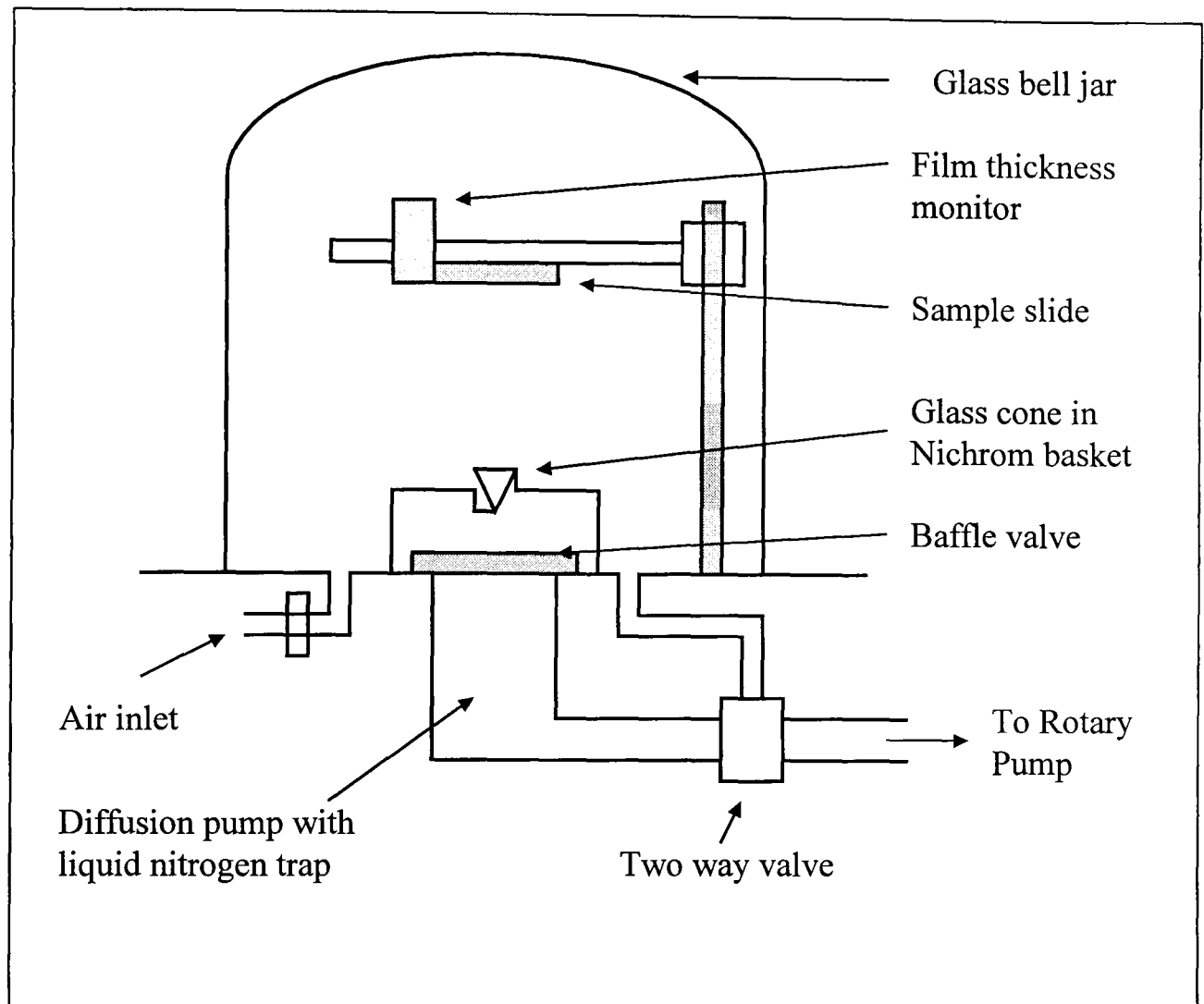
Fig 4.3:- Edwards E306 vacuum coating unit.
