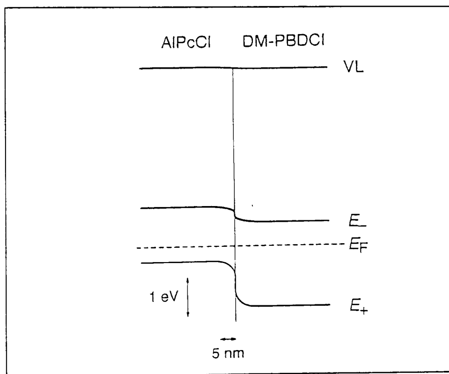
Fig 7.4: Diagram of MPCI/AlClPc junction proposed by Sato 143 .
