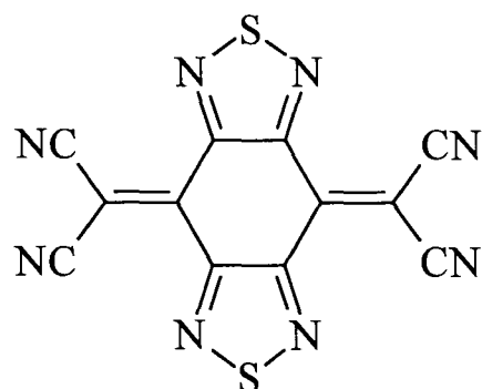
BTDA: bis (1,2,5-thiadiazolo) tetracyanoquinodimethane (sometimes referred to as BTDA-TCNQ)
