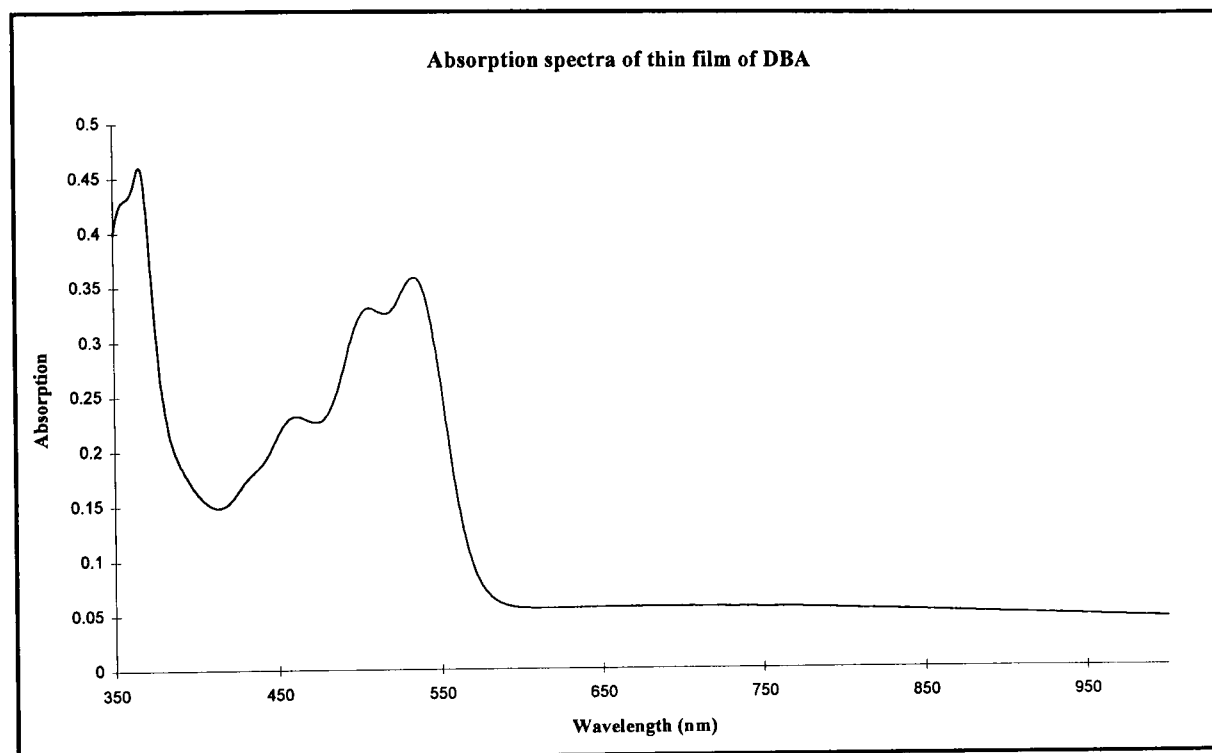
Fig 3.12: Absorption spectra of a thin film of DBA.
