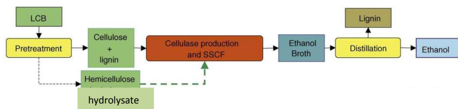
Figure 1.4: Flow diagram illustrating the concept of lignocellulosic biomass conversion to ethanol. Dotted lines represent optional process configurations (depends on pre-treatment used). LCB = lignocellulosic biomass, SSCF = simultaneous saccharification and co-fermentation process. Taken from Margeot et al. (2009).
