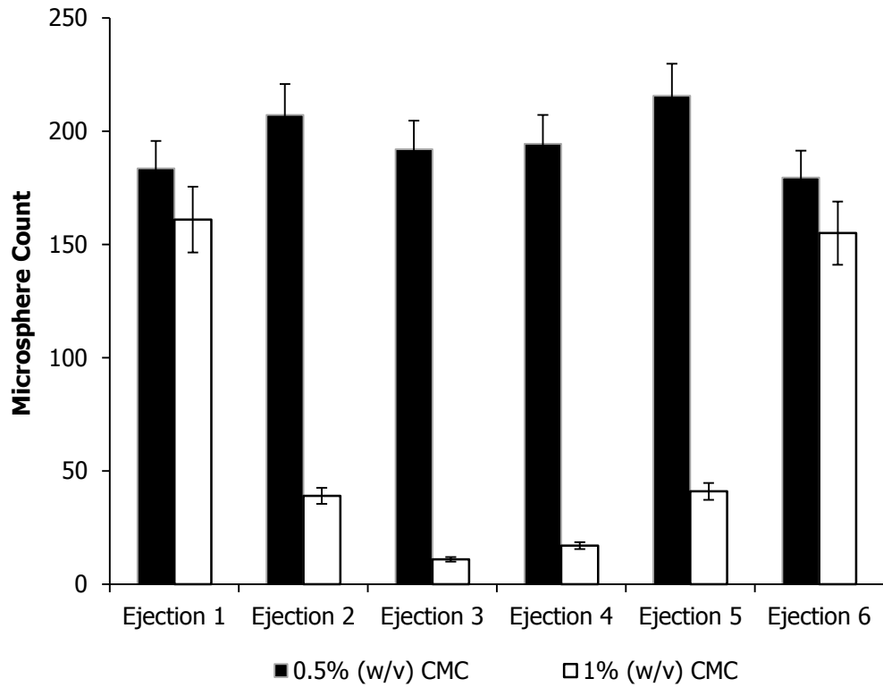
Figure 3.28 – ‘100 μm’ PLGA microsphere numbers as measured by light blocking for exemplar microinjection-based delivery conditions to illustrate the ability of the technique to distinguish between consistent and inconsistent delivery. Six series of six repeated ejections of 20% (w/v) suspension (1 μL per ejection) were performed through a 20 G needle using either 0.5 or 1% (w/v) CMC as the suspension fluid. Means are plotted with error bars showing the ‘process variability’.
