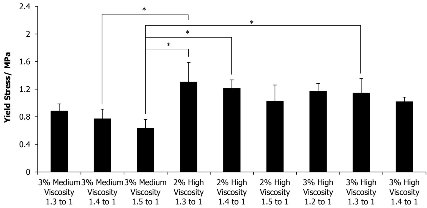
Figure 5.10 – Yield stresses for bioplotting PLGA-PEG microparticulate scaffolds as assessed by unconstrained compression testing (n = 3). PLGA-PEG microparticles were suspended in a variety of aqueous carriers at a variety of carrier:solid (v:w) ratios for bioplotting into cylindrical PTFE moulds. Samples were tested after 24 hours sintering. Error bars show one standard deviation and statistically-significant differences are denoted by (*).
