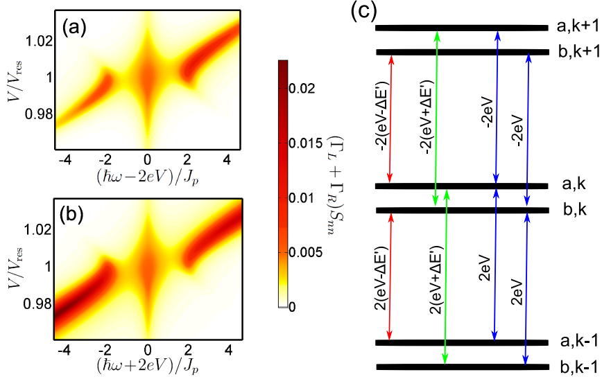
Figure 3.10: S_{n^{(1)}}(\omega) in the vicinity of the p = 1 resonance (a) and (b) show the spectrum at frequencies around \hbar\omega = \pm 2eV respectively. A schematic illustration of the processes giving rise to the spectral features is shown in (c). This illustrates the inter-doublet transitions and the corresponding frequencies of the features they give rise to.
