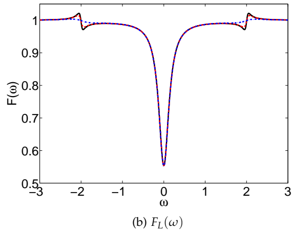
Figure D.4.: Frequency dependent Fano factor between the dots (a), and through the left junction (b). For all curves the parameters are \epsilon = 0 , \Omega = 1 , \Gamma = 0.1 , T = 10 . The curves show different couplings to the thermal bath. These are given by \gamma = 0 (black, solid line), \gamma = 1 \times 10^{-3} (red, dashed line) and \gamma = 1 \times 10^{-2} (blue, dotted line)
