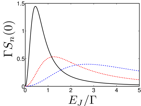
Figure 3.2.: Zero frequency charge noise S_n(0) as a function of E_J/\Gamma for various detunings, close to the JQP resonance. The solid, black line is \delta = 0 , the dashed, red line is \delta = \Gamma and the dotted, blue line is \delta = 2\Gamma .
