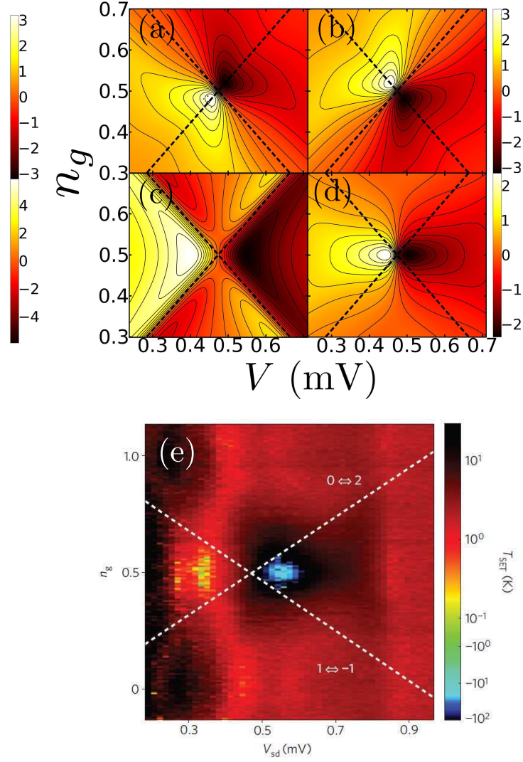
Figure 4.8.: Contributions to the inverse temperature (in K^{-1} ) from particle currents in (a) left, 1/T_L , and (b) right, 1/T_R , junctions; (c) contribution from the charge noise, 1/T_n and (d) total inverse temperature, 1/T_{BA} . Dashed lines indicate the two Cooper-pair resonances, which overlap at the DJQP resonance. For comparison, in (e) we reproduce the measured results, from Ref. [8], for the effective temperature of the oscillator due to the SSET.
