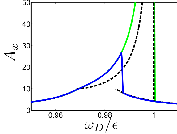
Figure 5.11.: Comparison of the numerical results to those obtained from the self-consistency expression. The solid green and blue lines show the numerical results for forward and backward frequency sweeps respectively. The black, dashed line shows the stable analytic solutions. The parameters are the same as Fig. 5.9.
