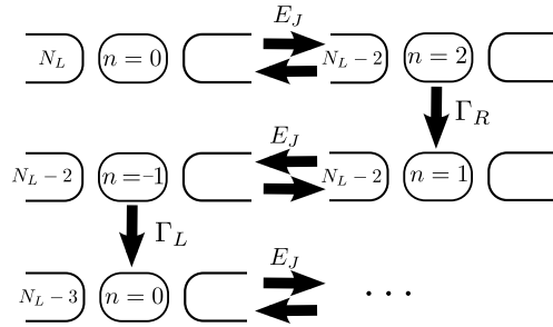
Figure 2.6.: The DJQP cycle. Quasiparticle decays and Cooper-pair tunnelling occurs at both junctions.
