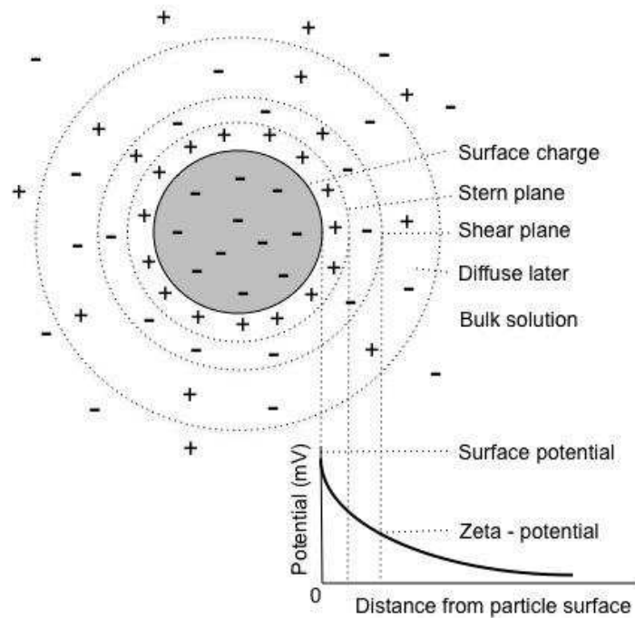
Figure 4.23 Zeta potential-potential difference as a function of distance from particle surface (adapted from BeckmanCoulter, Inc., 2010)
